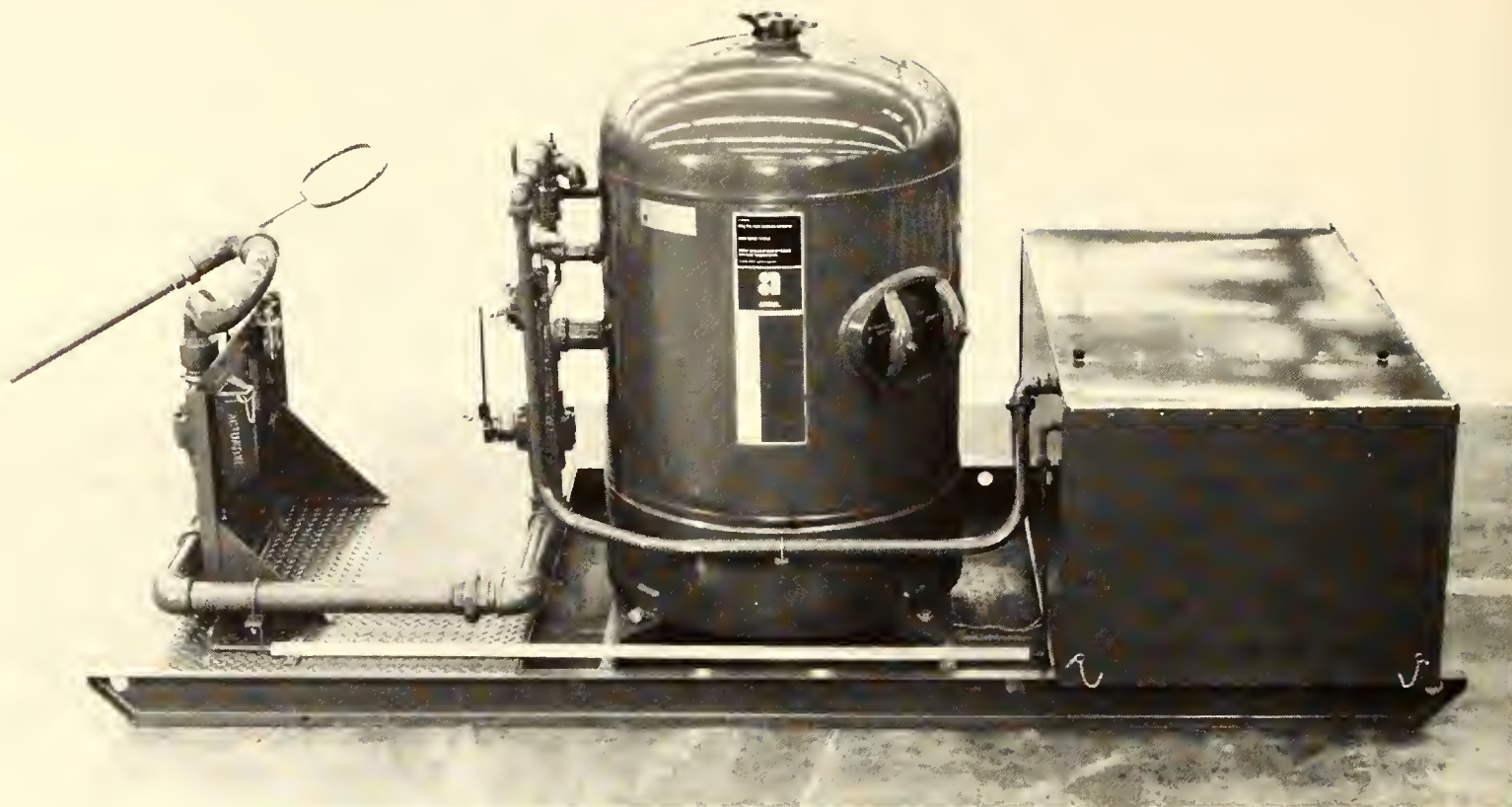
Figure 9.26. Typical skid-mounted dry chemical deck unit. (Courtesy Ansul Company)
