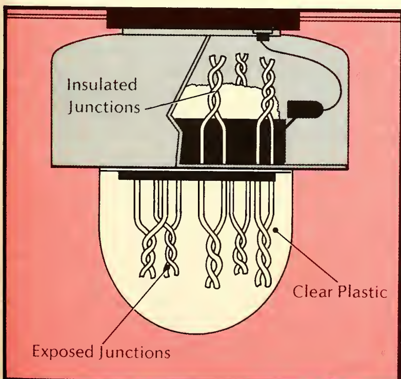
Figure 6.7. Thermoelectric spot rate-of-rise detector, with its two sets of junctions of dissimilar metal wires.
