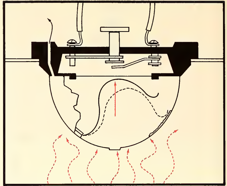
Figure 6.8B. The fixed-temperature device is a spring that is released when a fusible metal melts. The spring pushes up on the diaphragm and the contacts to transmit the alarm.
