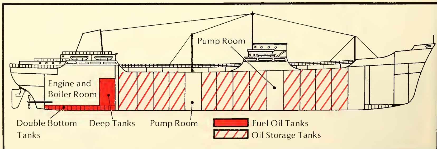
Figure 5.13. Location of liquid cargo and bunker tanks aboard tanker vessel.
