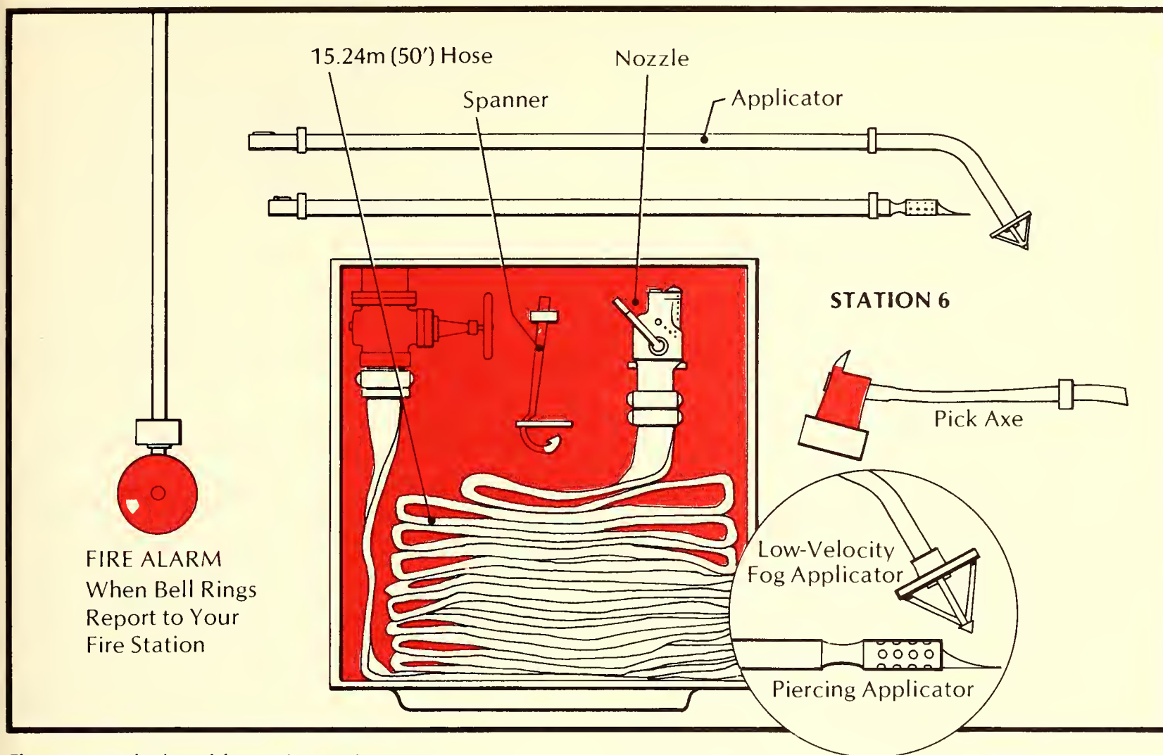
Figure 9.5. Shipboard fire station equipment.
