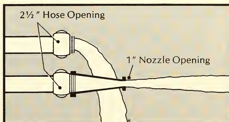
Figure 7.5. The taper greatly increases the velocity of the water coming from the nozzle.
