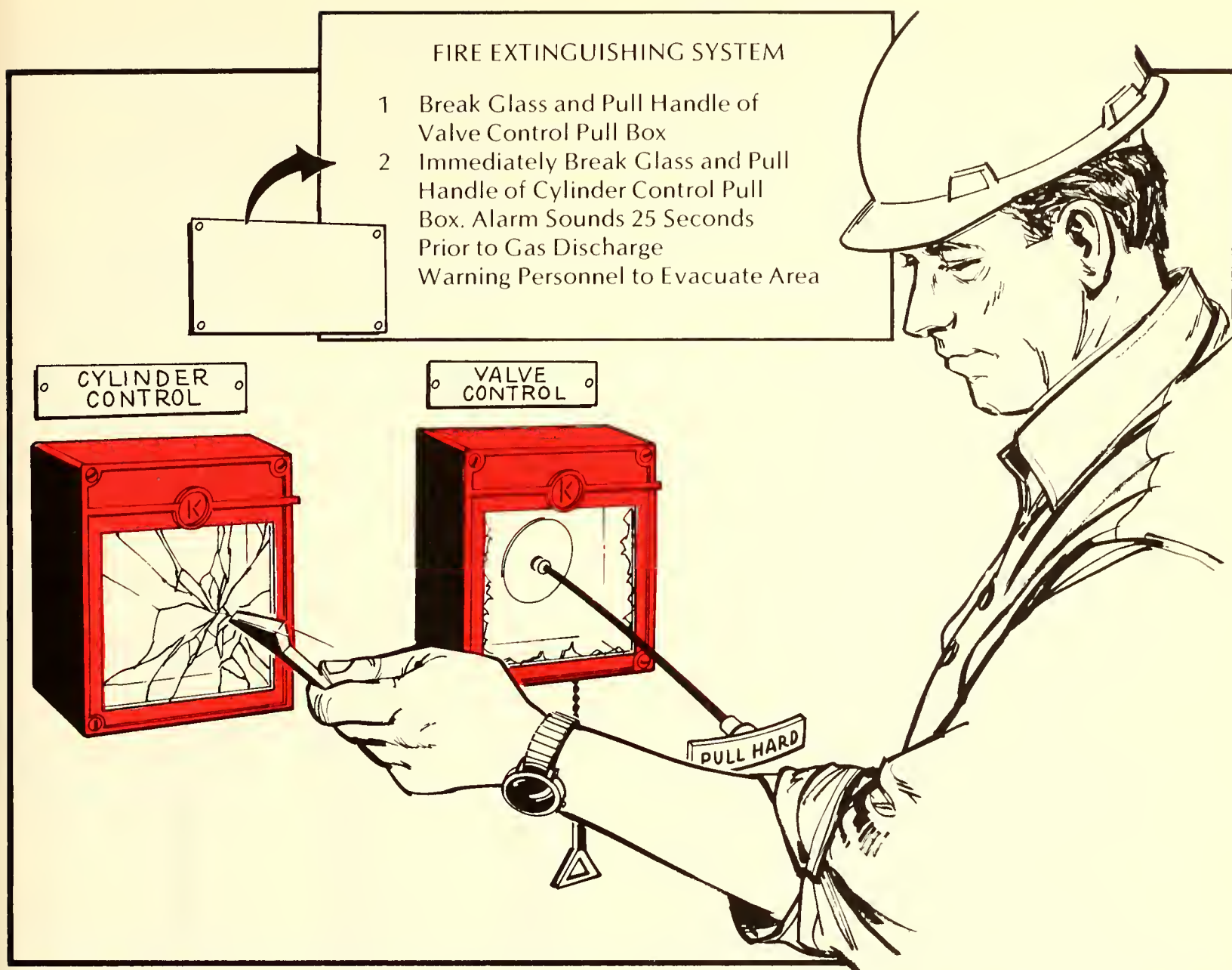
Figure 9.20. The pull cables used to activate the total-flooding CO 2 system. The cables must be pulled in the proper order (valve control first) as noted in the posted instructions.
