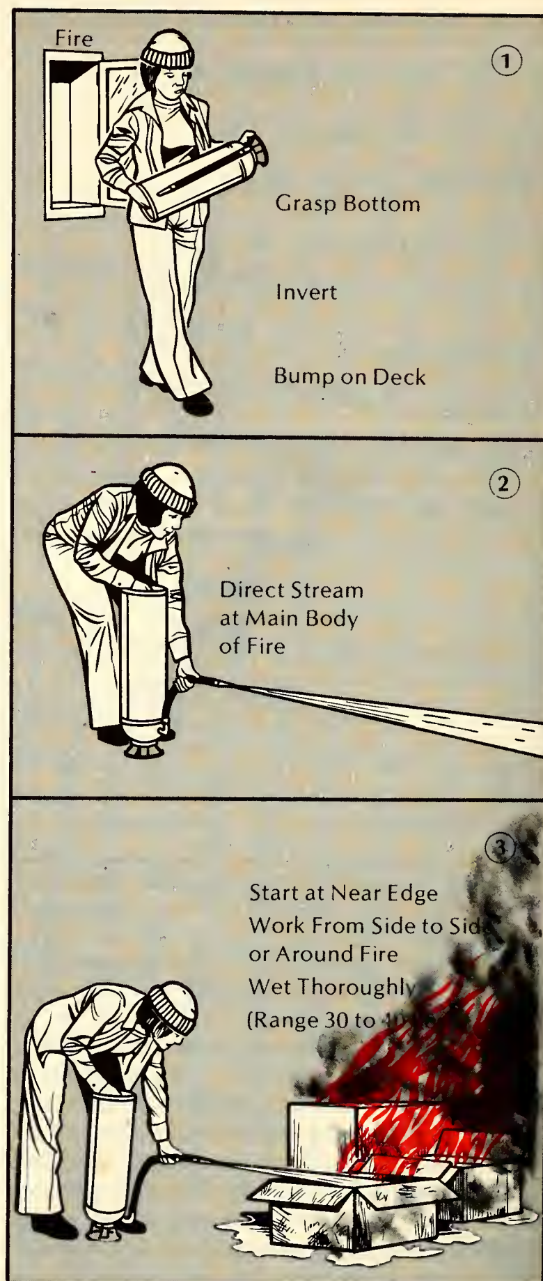
Figure 8.4. The cartridge-operated extinguisher is inverted and bumped on the deck. The stream is moved across the base of the fire.
