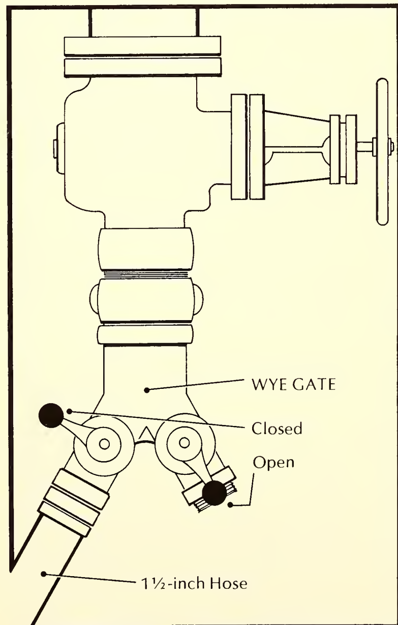
Figure 9.8. Wye gate attached to a hydrant outlet. Left, closed valve; right, open valve.
