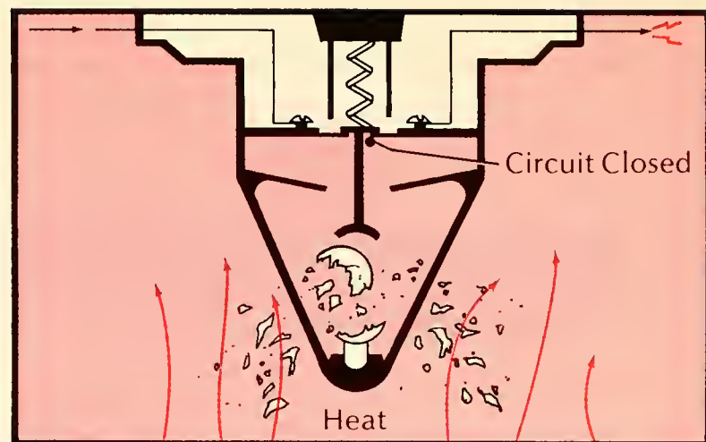
Figure 6.5B. At a preset temperature, liquid in the bulb has expanded enough to break the bulb. The plunger drops to complete the alarm circuit.
