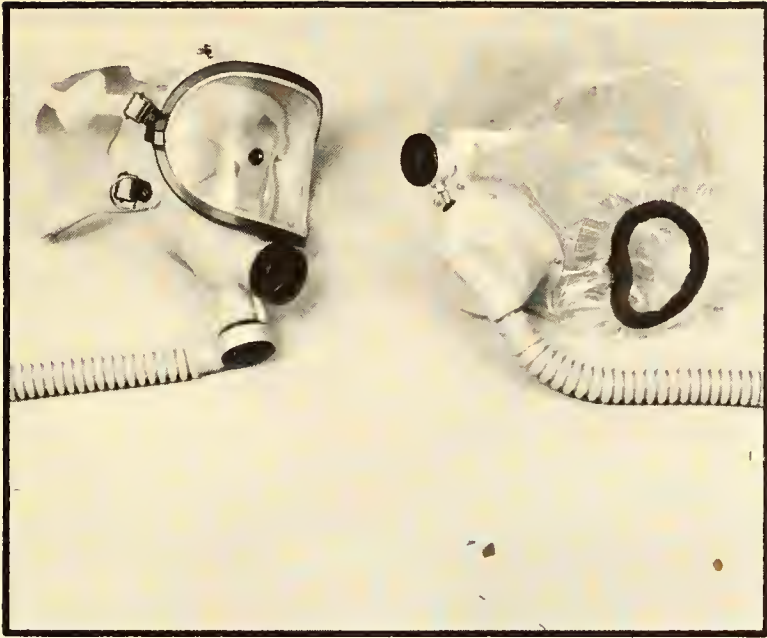
Figure 15.20. Standard facepiece (left) and polyurethane hood facepiece (right).
