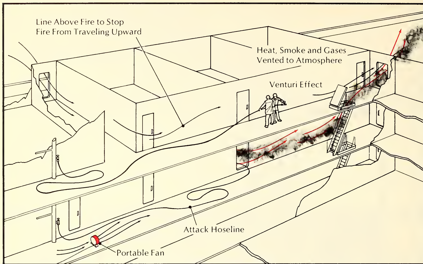
Figure 10.5. Combination venting. An airflow is created above the fire. It pulls combustion products up from the involved deck and out the doorway.
