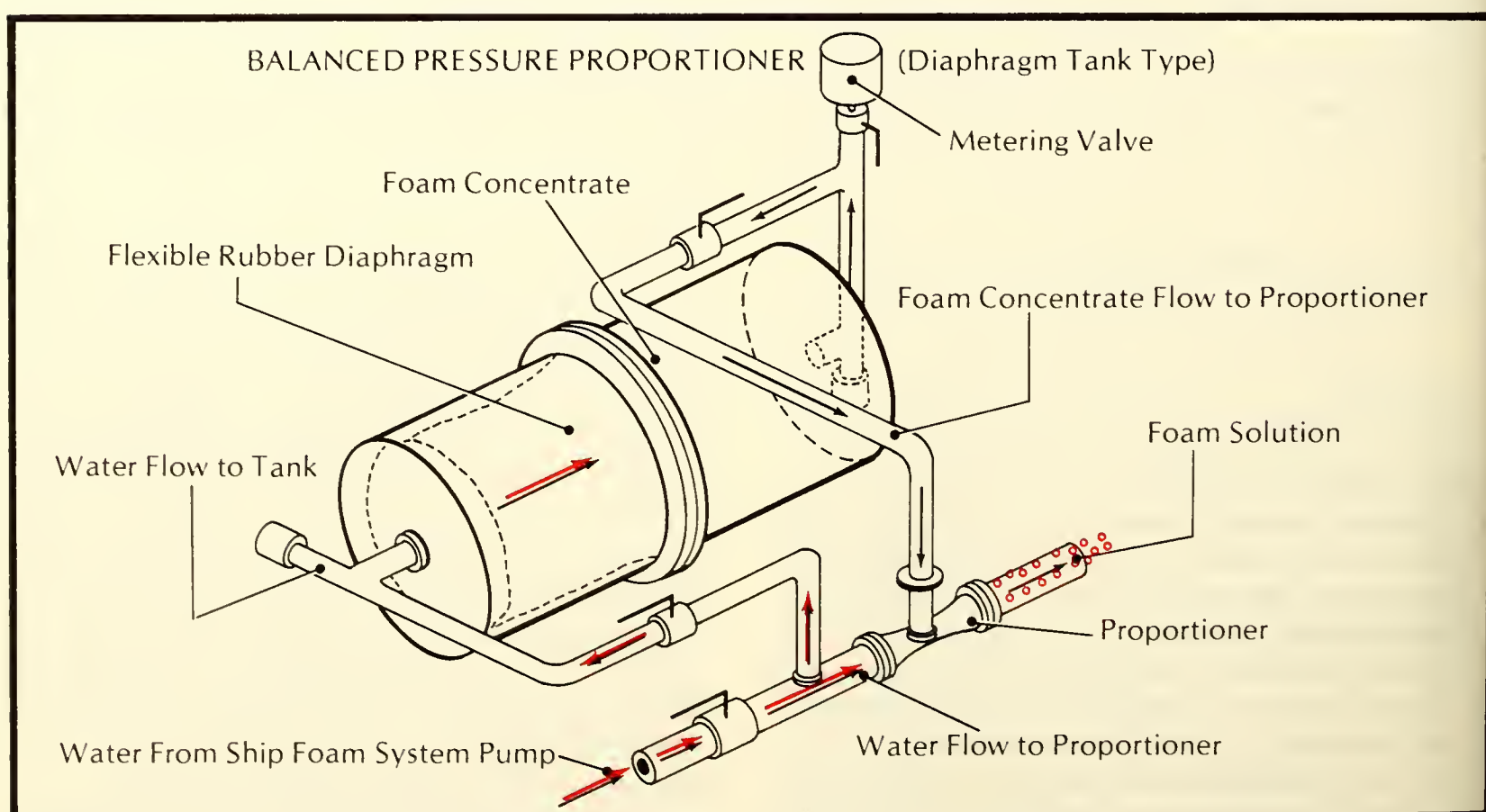
Figure 9.16. Schematic diagram showing the operation of a diaphragm-type foam concentrate tank. (Courtesy Rockwood System Corporation)
