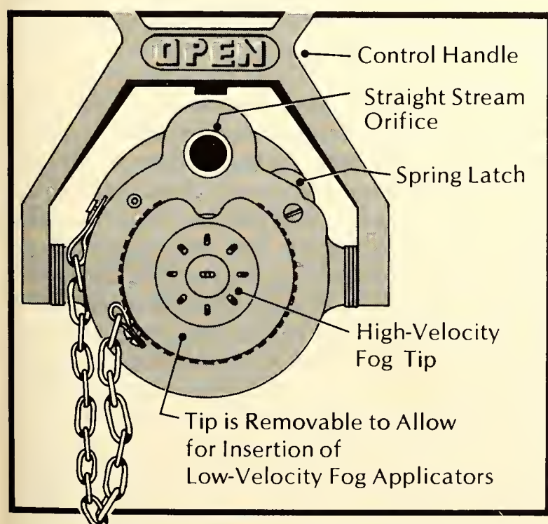
Figure 9.7. The outlet end of a combination nozzle.
