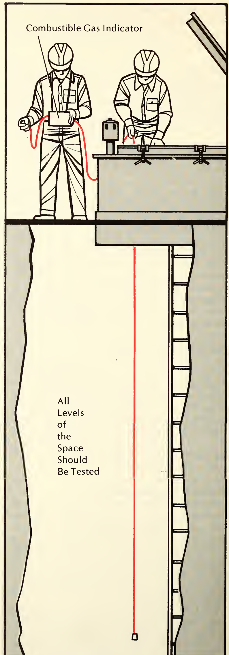
Figure 16.6. The sampling tube is inserted into the space to be tested for combustible gas. The instrument itself remains outside the space.
