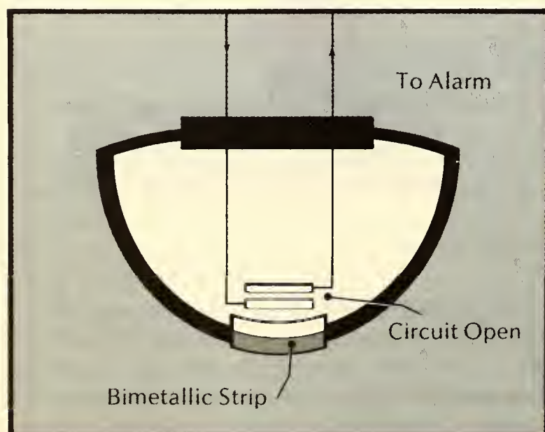
Figure 6.2A. The snap action bi-metallic disk. The disk at normal temperatures.
