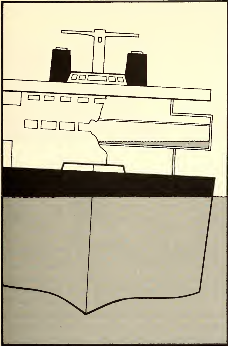
Figure 7.4. Water confined high on the ship has a detrimental effect on the ship's stability.
