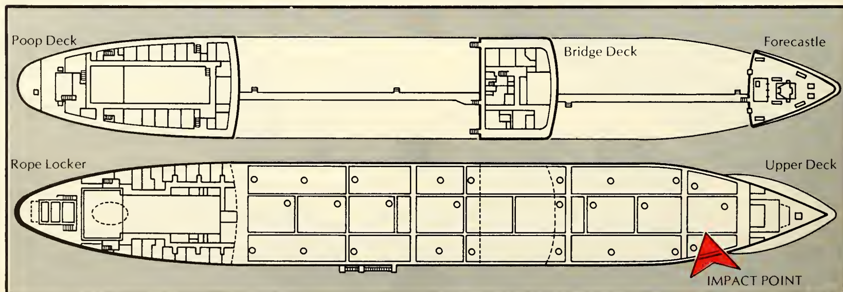
Figure 3.4. Superstructure and tank decks for the Alva Cape . Arrow marks the point of impact.
