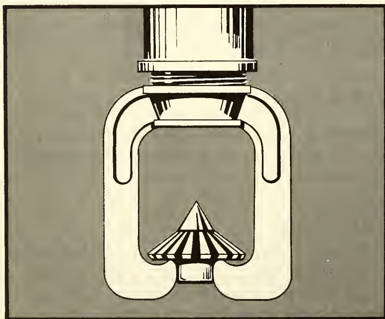
Figure 9.12. Typical spray head. There is no fusible link; the head is open at all times.
