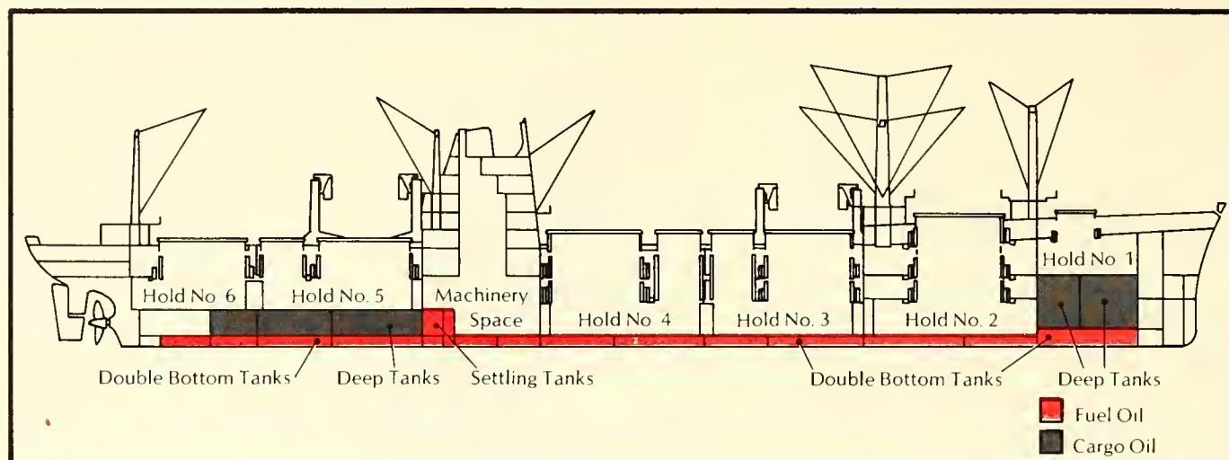
Figure 5.12. Location of liquid cargo and bunker tanks aboard dry cargo vessel.
