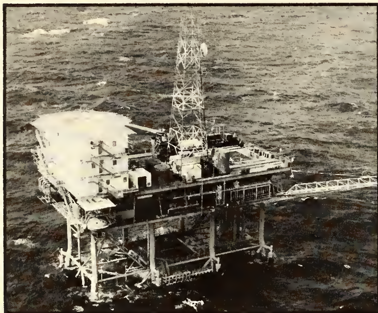
Figure 12.1. A fixed offshore unit of recent design. The platform is supported by a steel base fastened to the seabed.
