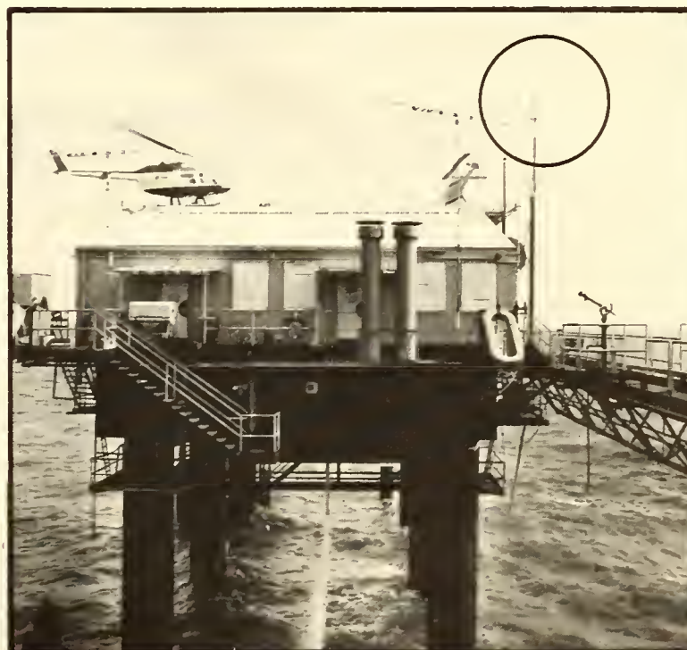
Figure 12.10. Monitor nozzles, positioned to reach the helicopter pad, can apply large volumes of water from a safe distance.
