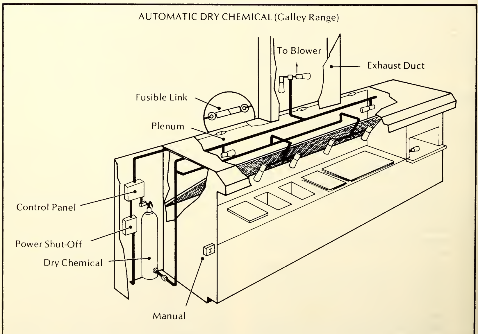
Figure 9.27. Typical automatic dry-chemical galley range system.
