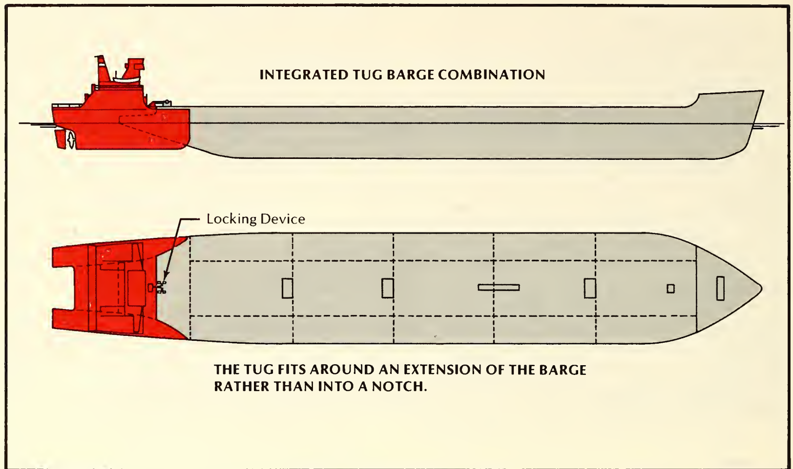
Figure 11.3. A modern integrated Tug Barge system.
