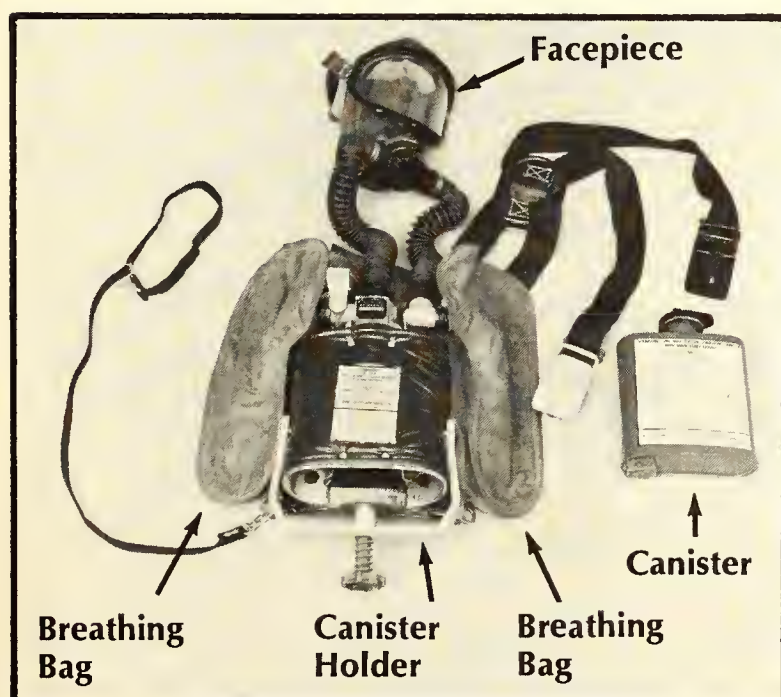
Figure 15.7. Self-generating canister-type OBA.
