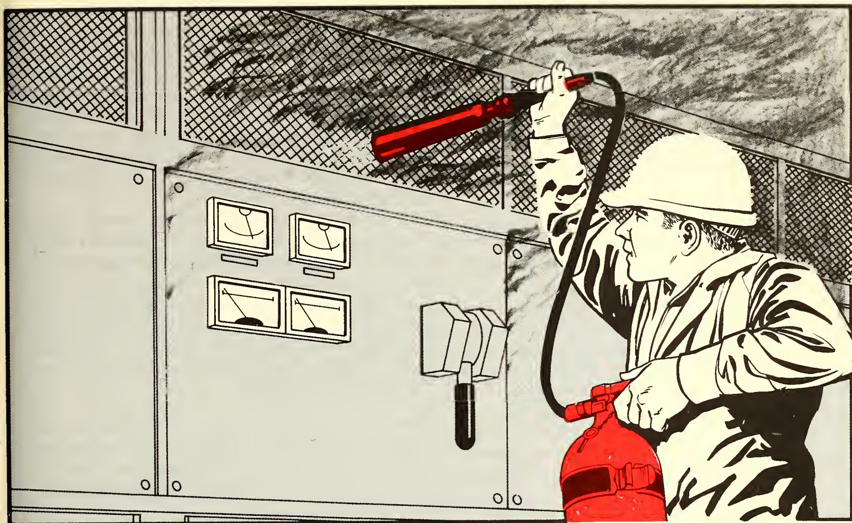
Figure 10.14. Fire in an enclosed electrical cabinet should be attacked with CO 2 or Halon. The agent should be directed into the unit through the cabinet vents.
