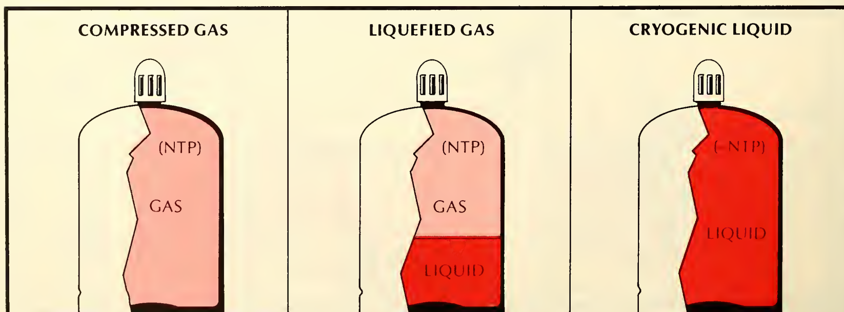
Figure 5.15. The differences among compressed, liquefied and cryogenic gases.
