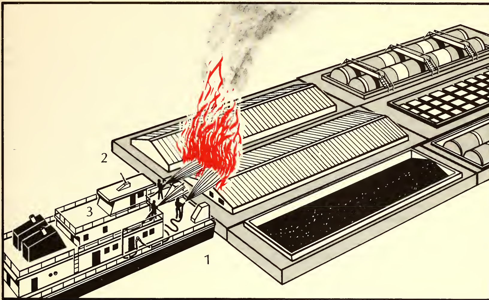
Figure 11.11. When fire threatens the tow vessel, it must be protected. Lines 1 and 2 attack the fire directly; line 3 protects firefighters and the tow vessel. Quick beaching of the tow is imperative.
