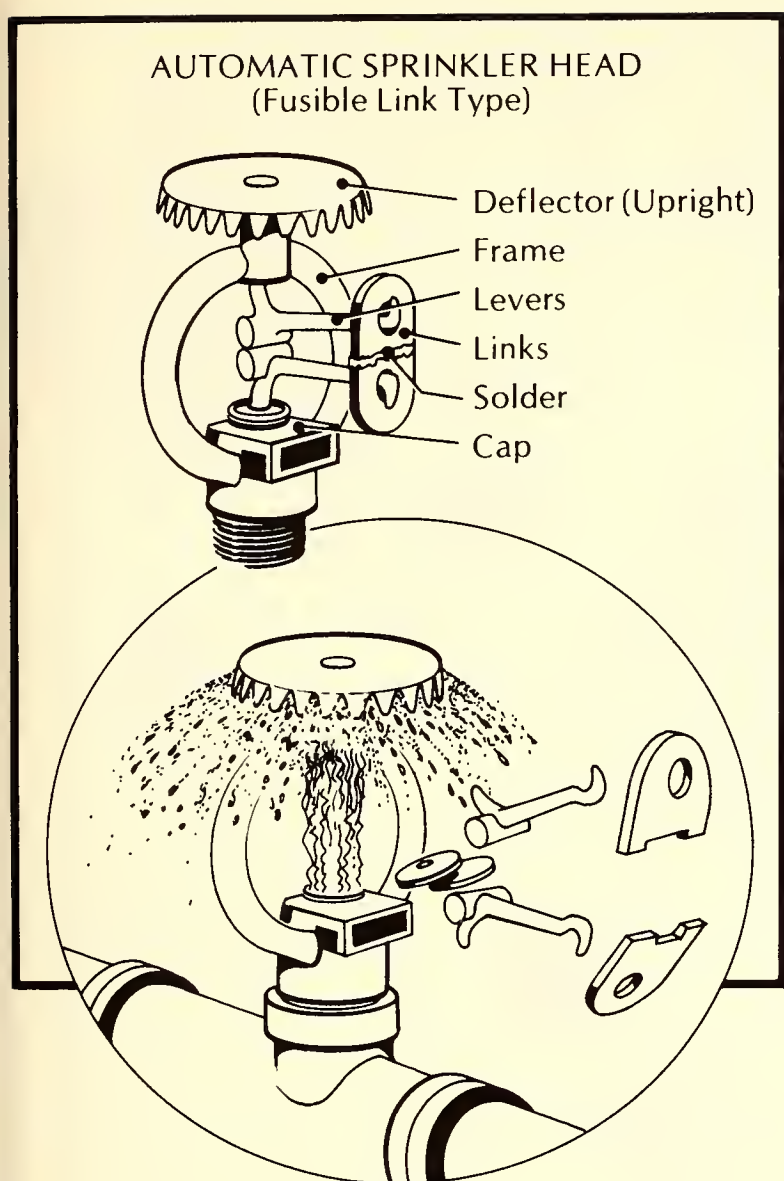
Figure 9.9. A. Heat from fire melts solder, allowing links to separate. B. The levers come apart and C. water pressure pushes the valve cap off the sprinkler outlet. D. Water flows up against the deflector, forming a spray that falls onto the fire.
