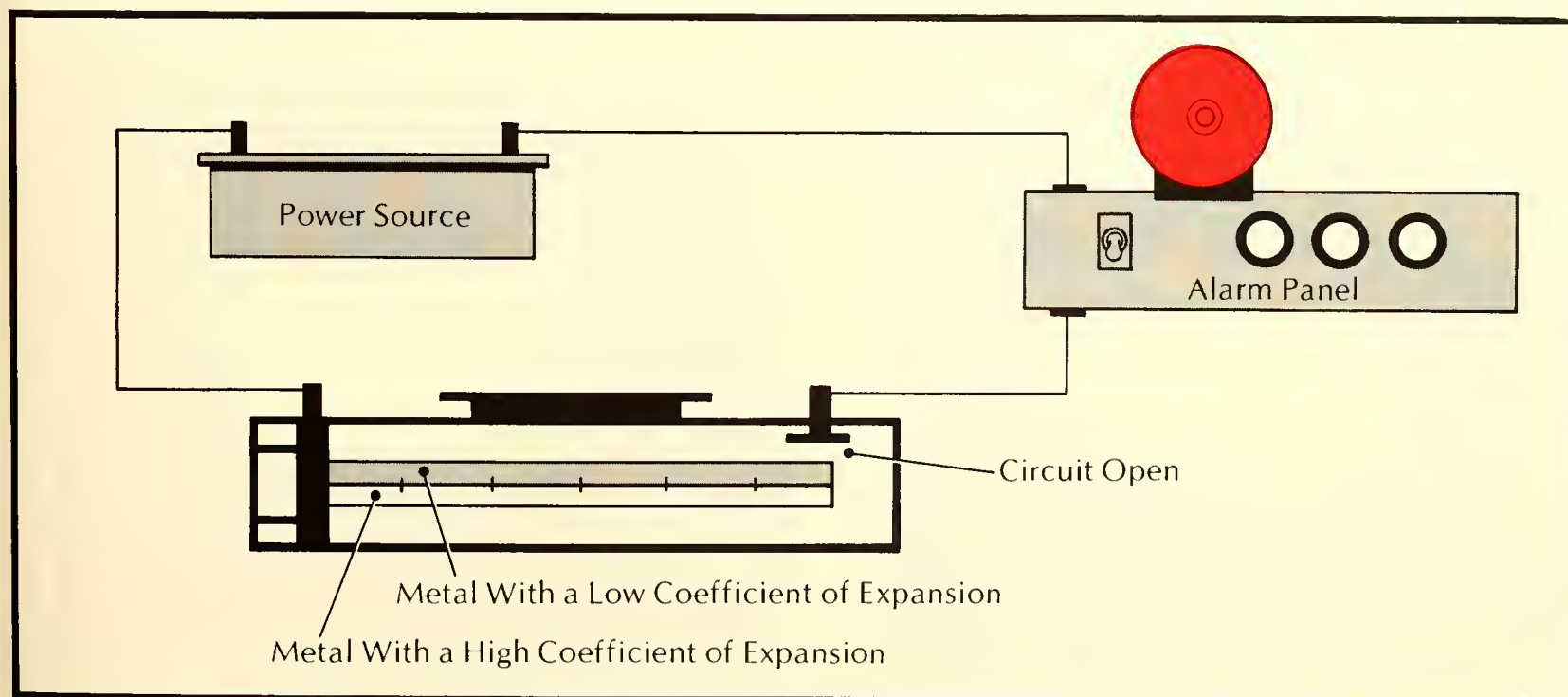
Figure 6.1A. The bi-metallic strip heat detector. At normal temperatures, the strip is straight.
