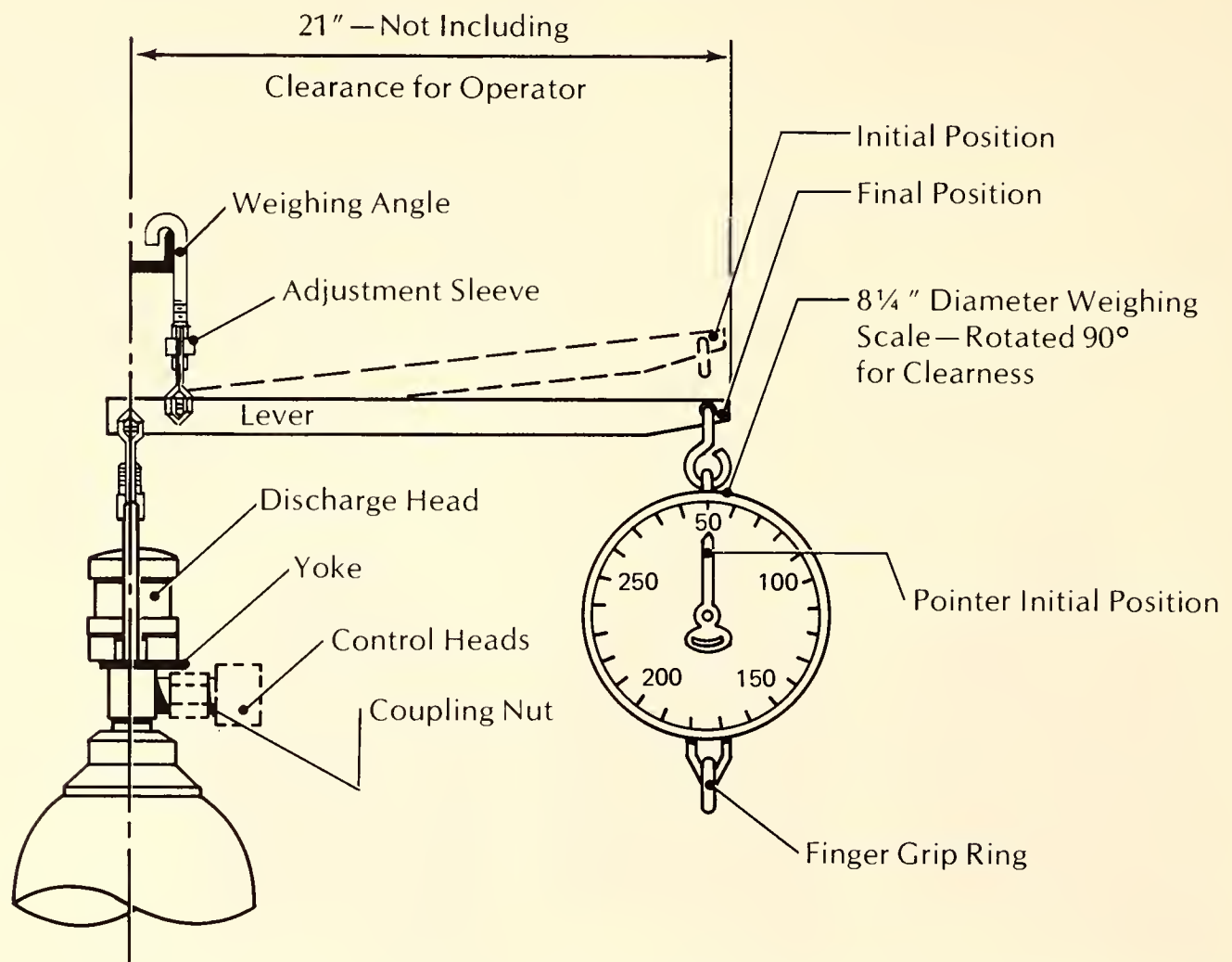
Figure 9.24. Carbon dioxide cylinder weigh bar and its use. (Courtesy Walter Kidde and Company)
