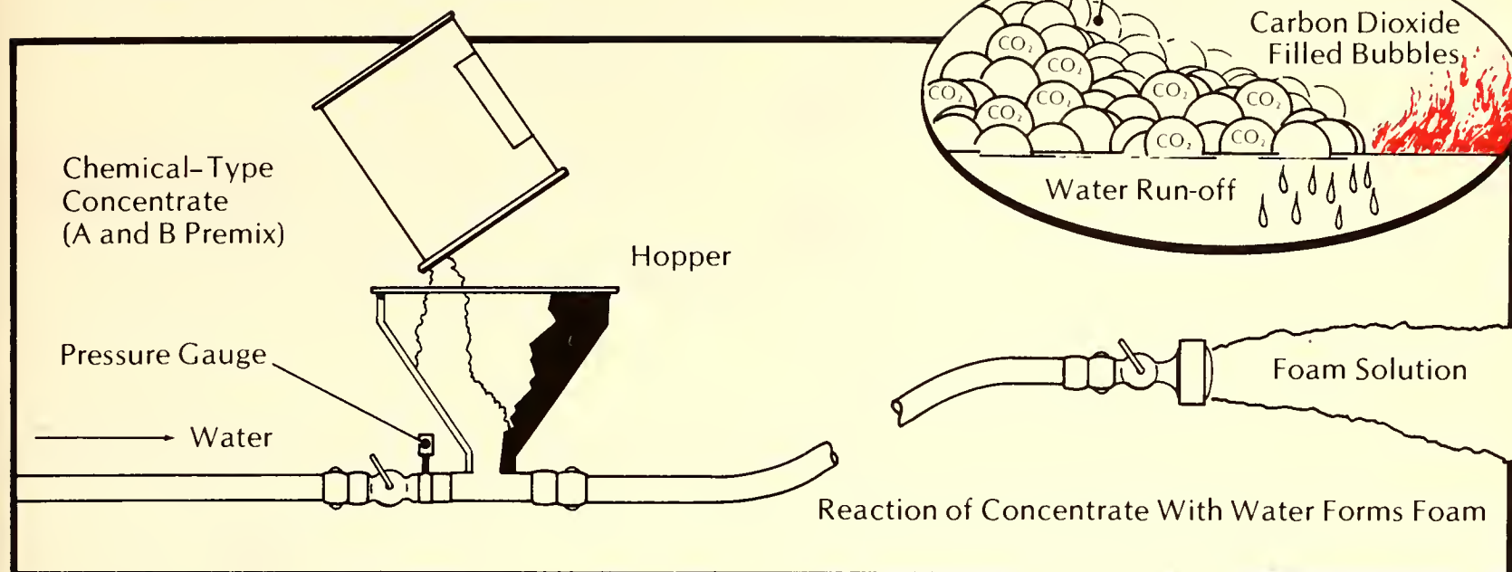
Figure 7.15. Production of chemical foam with a foam hopper.
