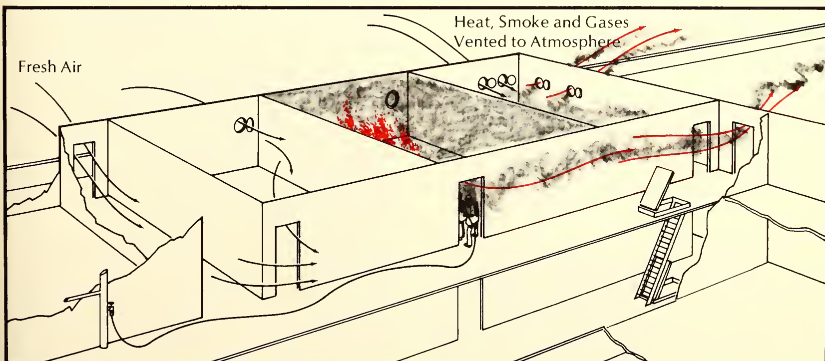
Figure 10.4. Horizontal ventilation. Fresh air entering through windward doorways and portholes pushes heat and smoke out leeward doorways and portholes.
