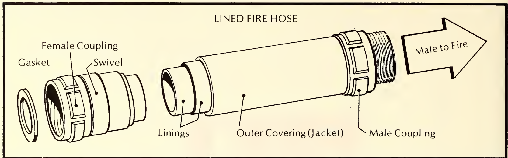
Figure 9.6. Lined fire hose and hose couplings.
