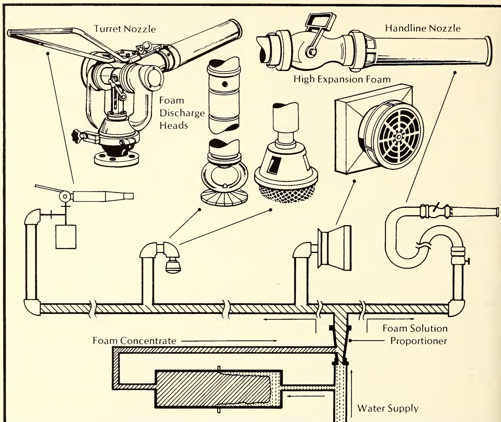
Figure 9.18. Fixed mechanical foam systems can supply turret and handline nozzles, foam discharge heads and high-expansion foam devices. (Courtesy Rockwood Systems, Inc.)
