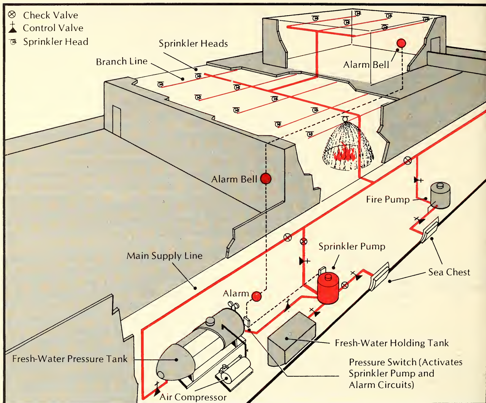
Figure 9.10. Shipboard automatic sprinkler system. The sprinkler pump is started automatically by a switch in the pressure tank.
