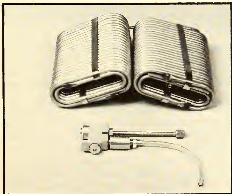
Figure 15.19. Air modules and flow regulation unit for a module-supplied, demand-type apparatus.
