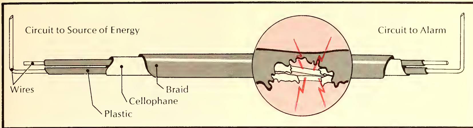
Figure 6.3. The thermostatic cable. The top wire is electrically energized; the bottom wire is not. At the activating temperature, the insulating material melts, allowing the two wires to touch and complete the alarm circuit.
