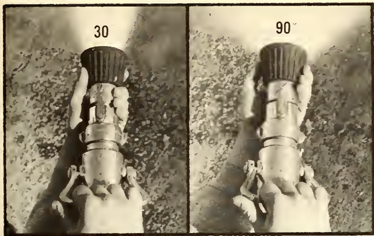
Figure 12.8C. The adjustable fog nozzle will deliver a 30° or 90° fog pattern as well as a solid stream.
