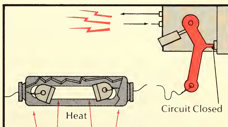
Figure 6.4B. When the link melts, the movable contact is free to complete the alarm circuit.
