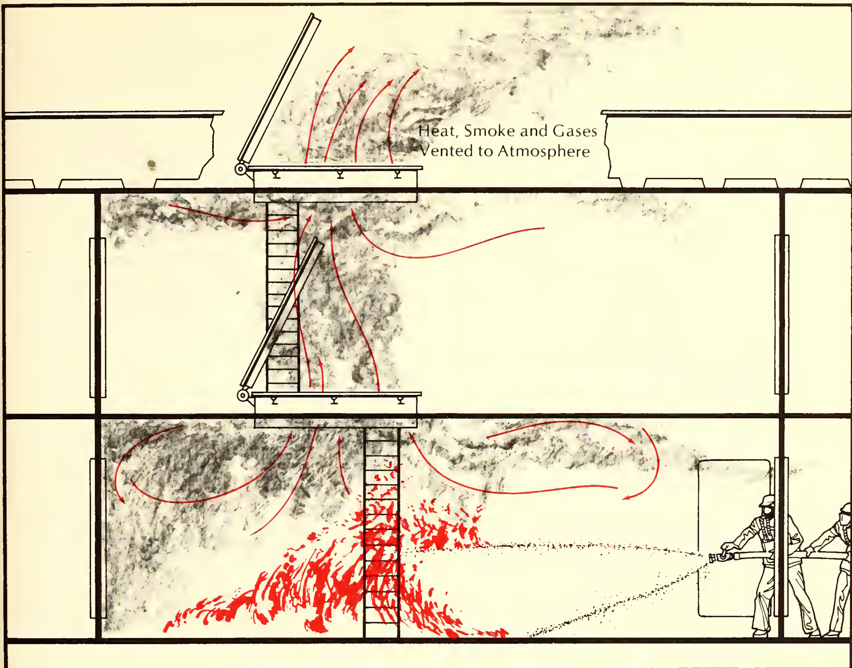
Figure 10.3. Vertical ventilation, directly upward from the fire to the atmosphere.
