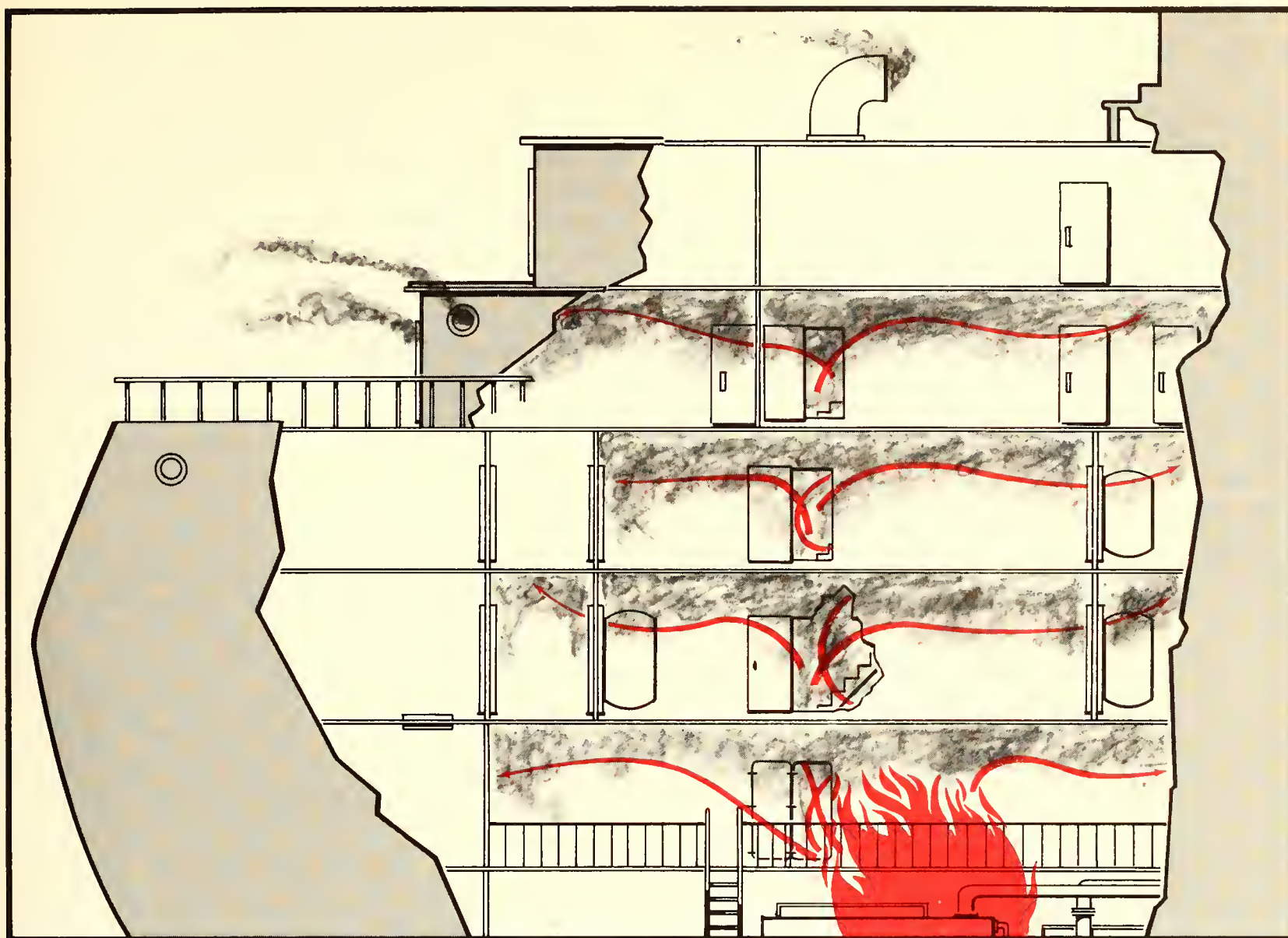
Figure 4.11. Convection carries heated air, gases and smoke upward through the ship. When vertical passage is blocked, they move horizontally.
