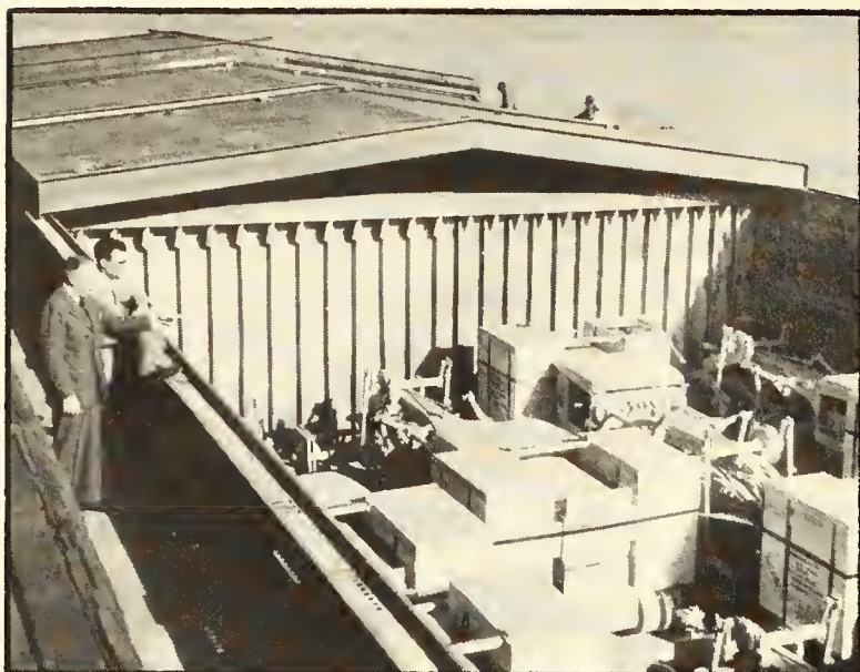
Figure 11.7. Typical covered dry-cargo barge with rolling weathertight hold cover. (Courtesy American Waterways Operators, Inc.)
