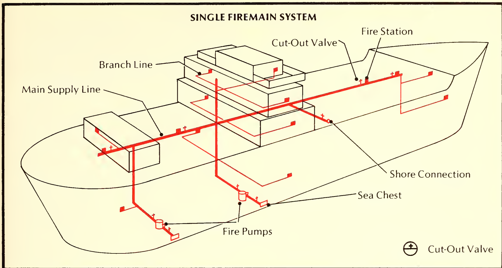
Figure 9.1. Typical single main system.
