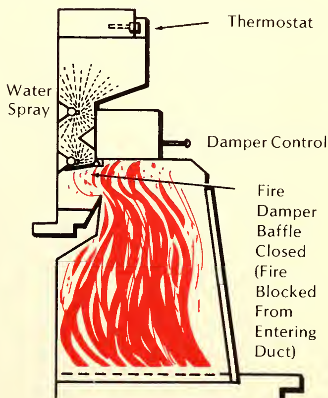
Figure 9.29. The fire damper system. A. Normal operation. B. During a fire. When the thermostat senses fire, the fire damper baffle is closed and the spray nozzles are activated. This keeps fire out of the ductwork. (Courtesy Gaylord Industries, Inc.)
