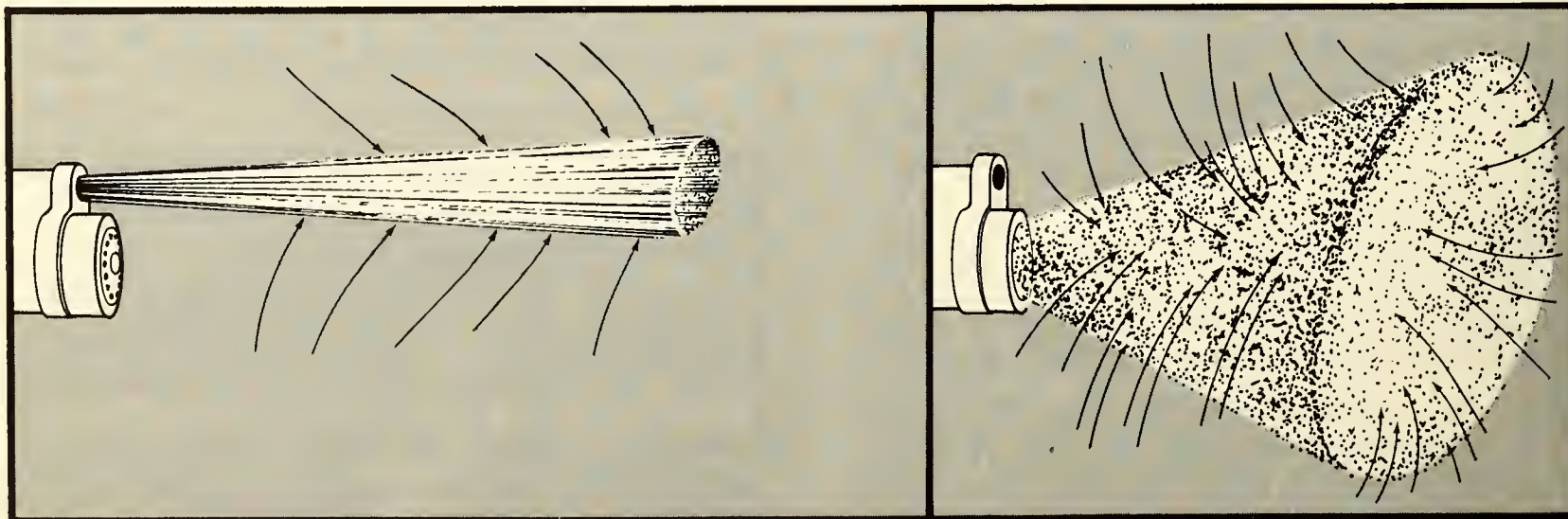
Figure 7.7. A. Straight stream. B. Fog stream. The fog stream droplets present a greater water surface area to the fire and can absorb more heat.
