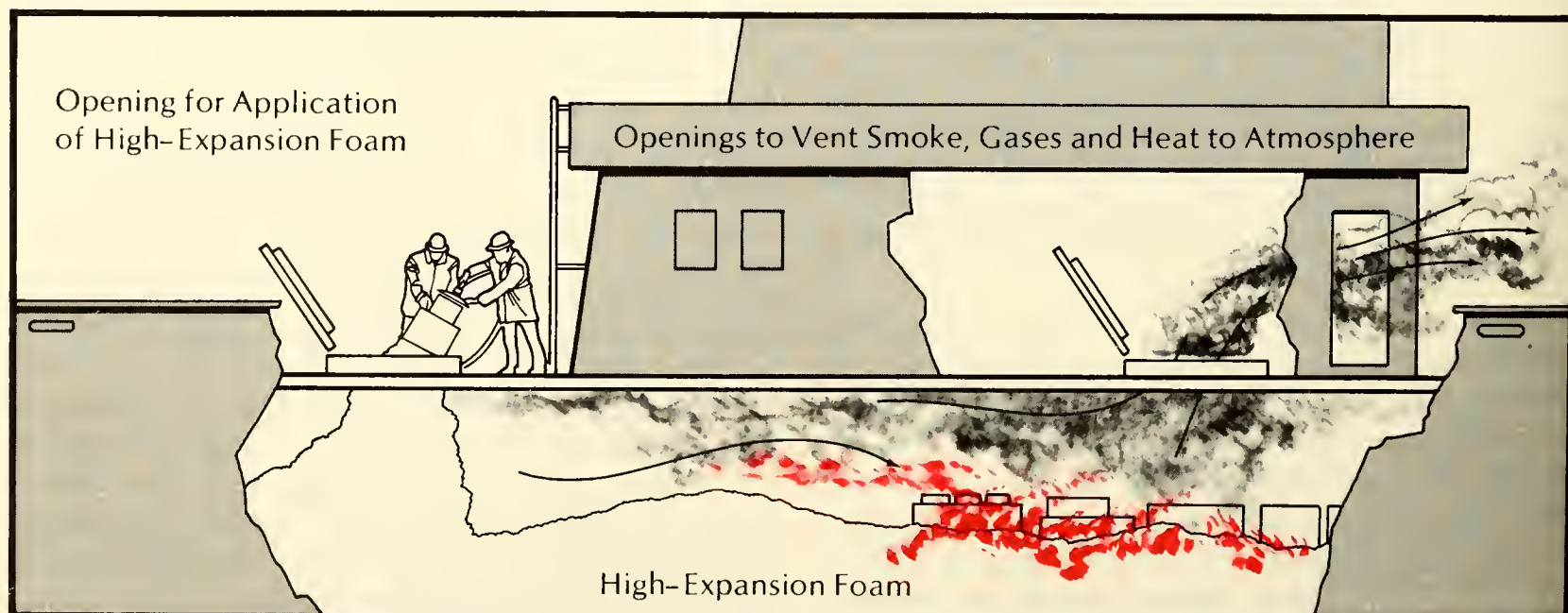
Figure 7.18. Flooding a cargo hold with high-expansion foam. Here, hatches are being used to apply the foam (left) and to vent the products of combustion including the hot steam that is produced (right).
