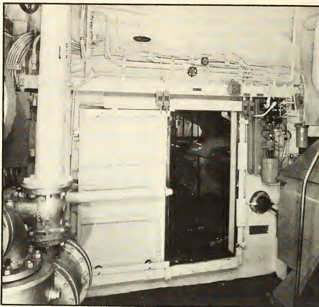
Figure 16.2. A horizontal watertight class A (and class 3) door separating the engine room from the shaft alley. (Courtesy Walz and Krenzer Inc.)
