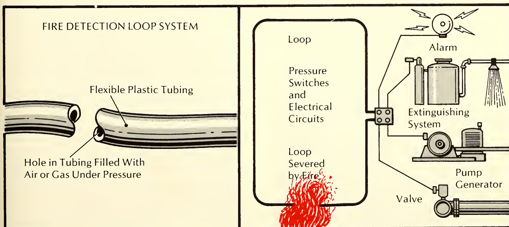
Figure 12.3. Fire detection loop system. A. Plastic tubing whose hollow core is filled with gas or air under pressure. B. When the tubing is severed, the pressure is lost. The reduced pressure allows switches to activate emergency equipment, including alarms, extinguishing systems, generators and product control valves.
