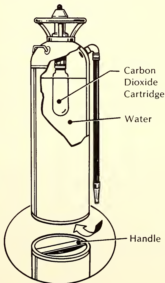
Figure 8.3. Cartridge-operated water extinguisher used for class A fires only.
