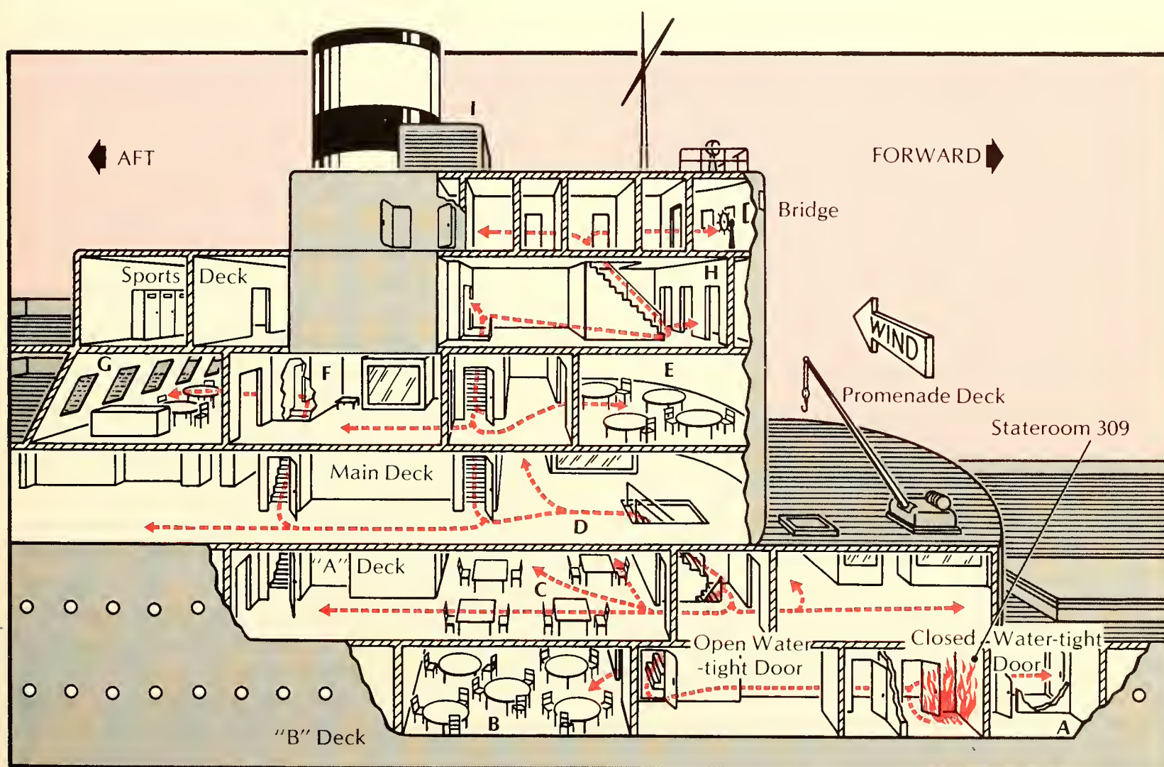
Figure 3.2. Cutaway view of part of the Rio Jachal . The arrows show the extension of the fire from stateroom 309 (the site of the fire) to the bridge.
