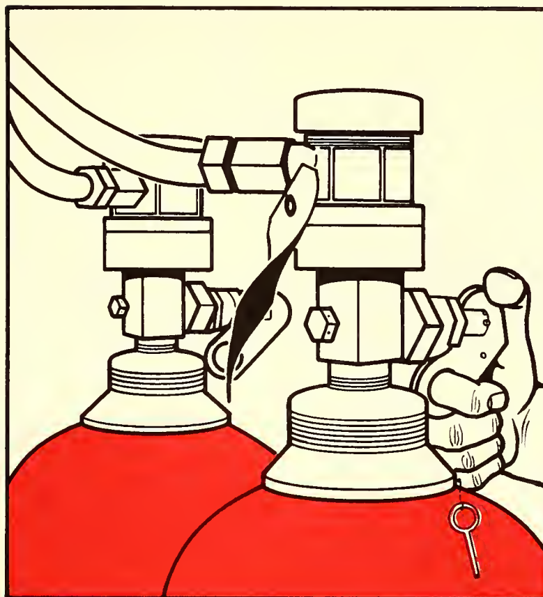
Figure 8.16. The activating lever on one CO 2 cylinder is operated after the locking pin is removed.
