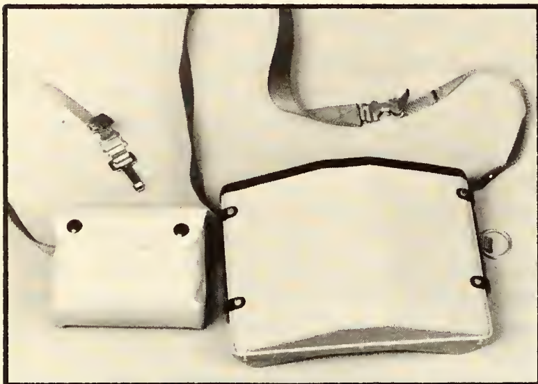
Figure 15.22. Harness and carrying case for the module-supplied apparatus.
