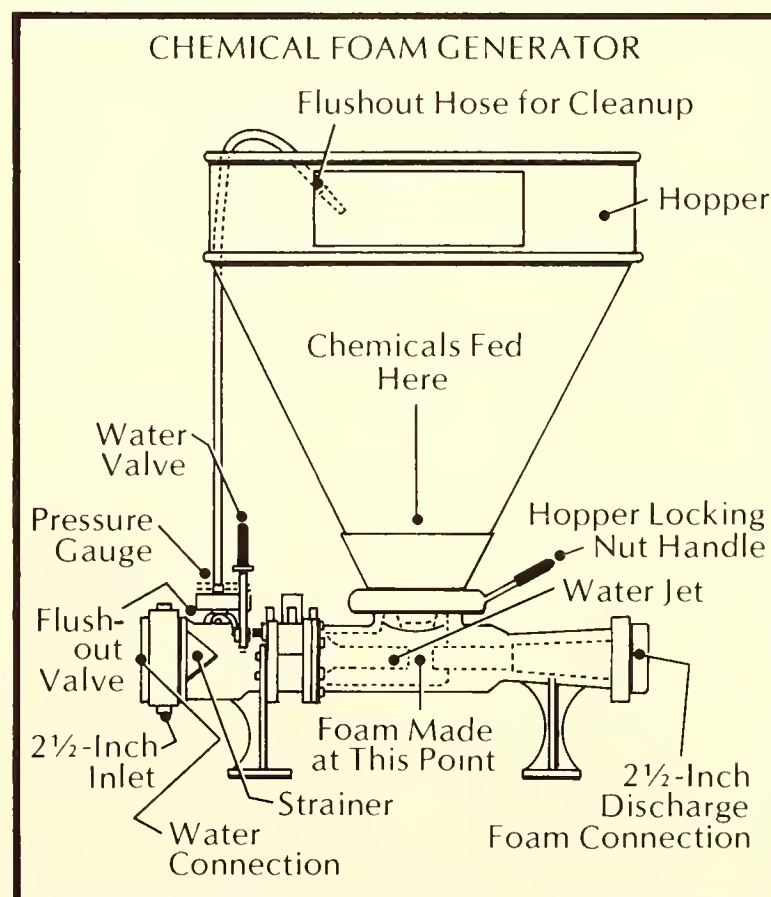
Figure 9.14. Continuous-type chemical foam generator. A. The generator is connected to a hoseline or piping to the fire main. B. Foam chemicals are discharged into water flowing through the bottom of the generator. C. Chemical foam is produced downstream of the generator.
