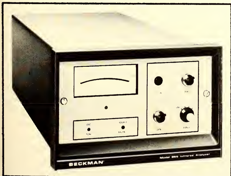
Figure 6.17. Nondispersive infrared gas analyzer. The meter indicates the concentration of gas in each sample as it is being analyzed.
