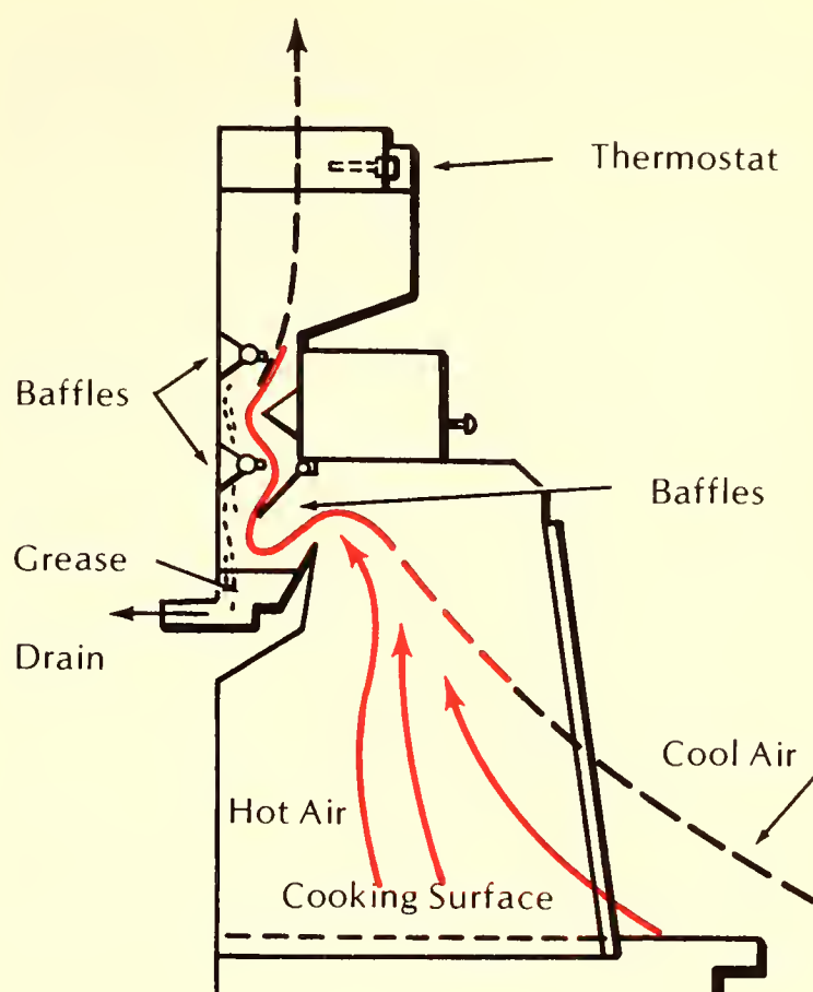
Figure 9.28. Galley ventilator washdown system. During normal operation, grease-laden air passes around a series of baffles, where the grease is removed.
