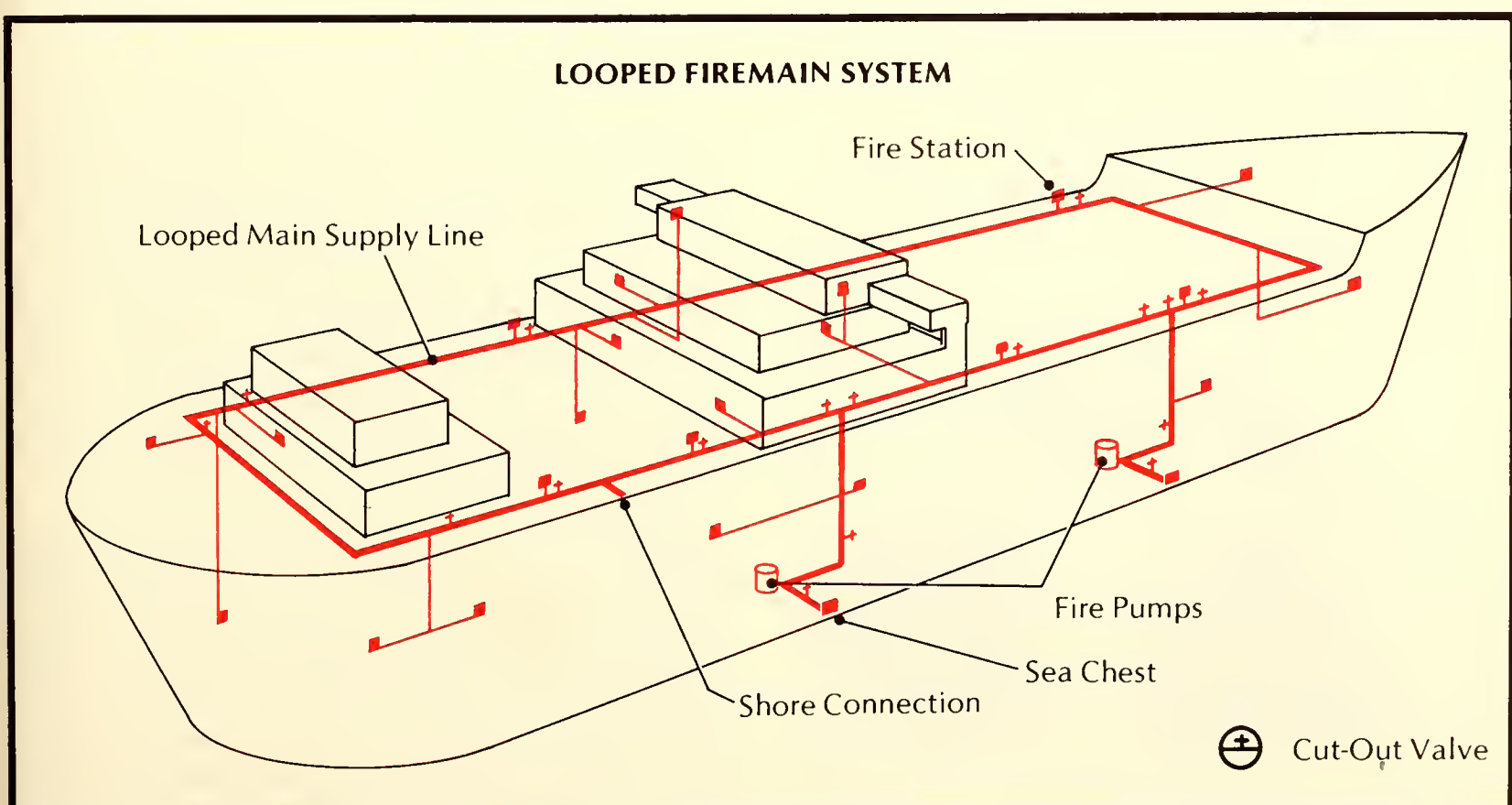
Figure 9.2. Typical horizontal loop fire-main system.
