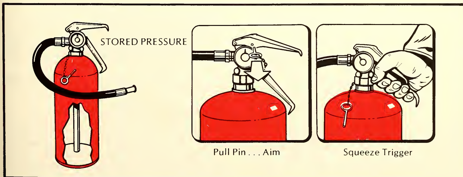
Figure 8.10. Operating the stored-pressure dry-chemical extinguisher.
