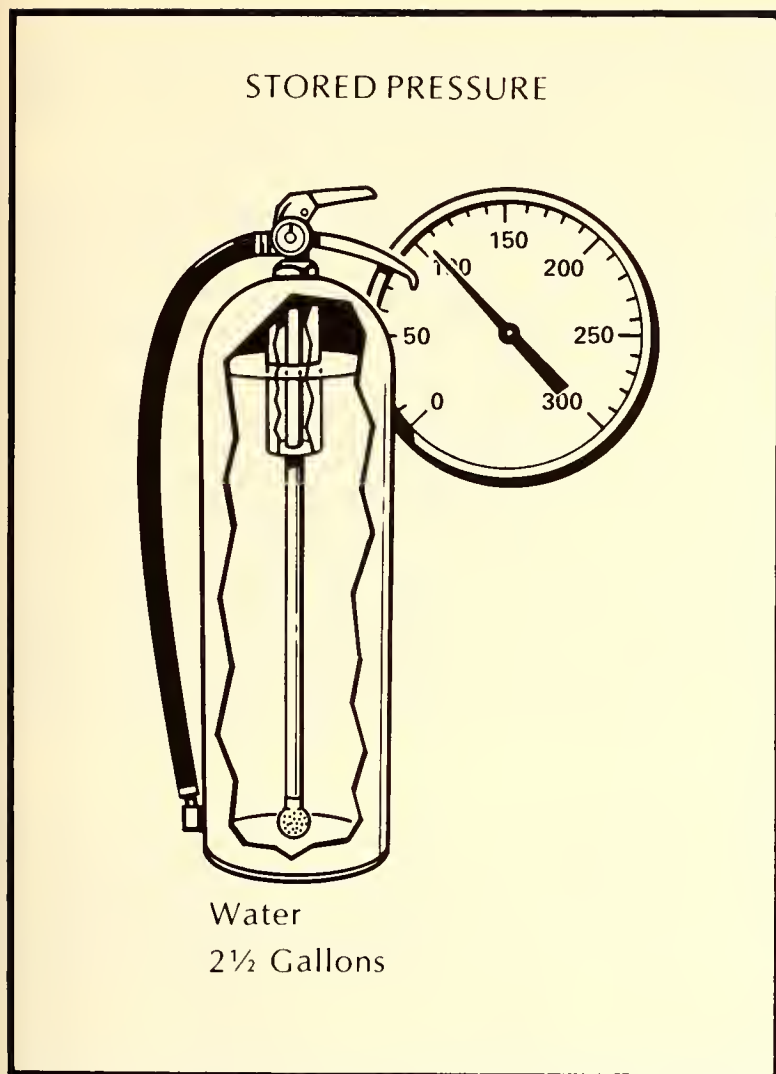
Figure 8.5. Stored-pressure water extinguisher used for class A fires only.
