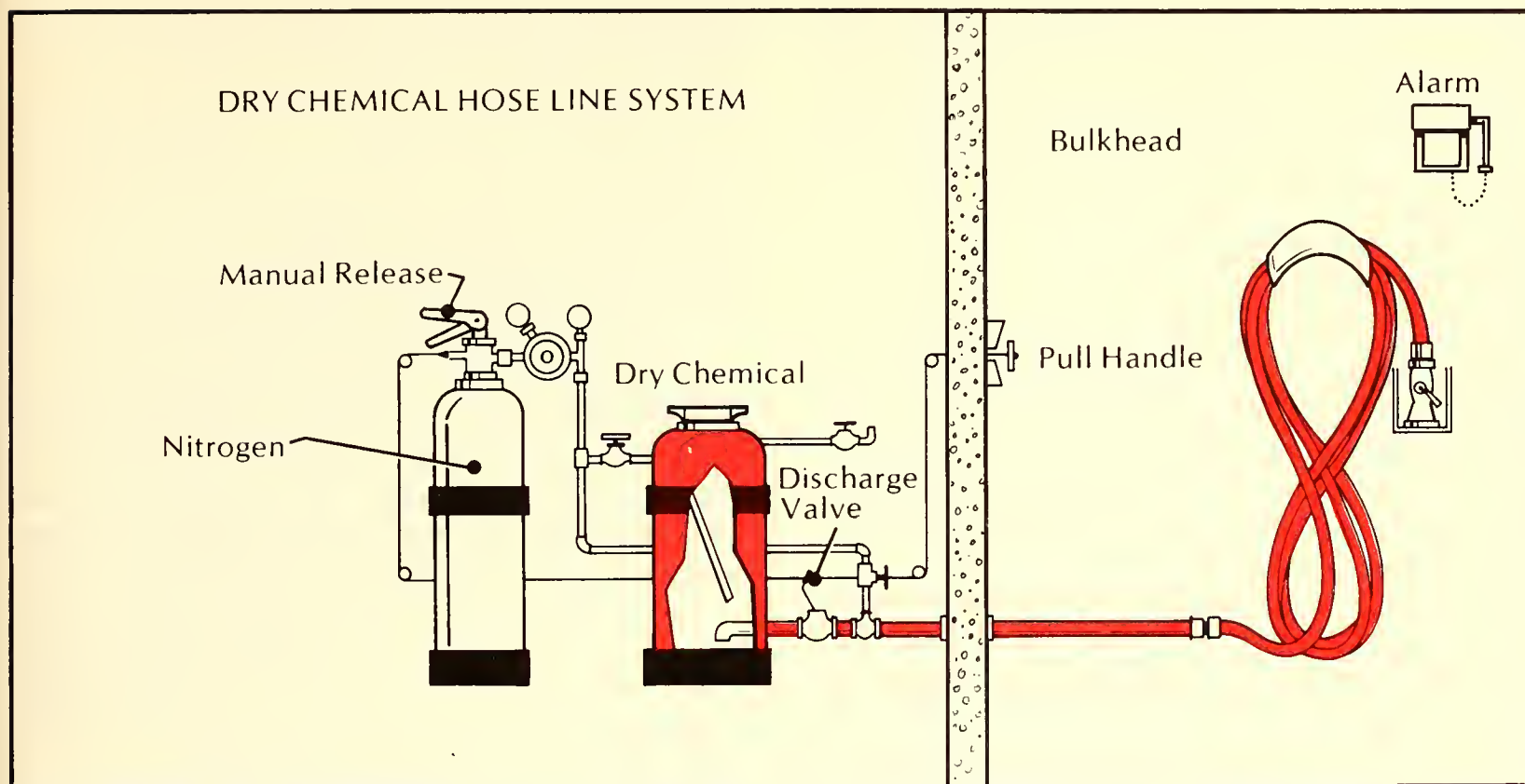
Figure 8.19. Dry chemical hose system with a remote-cable activating device. In some installations, the entire system is located in one space.
