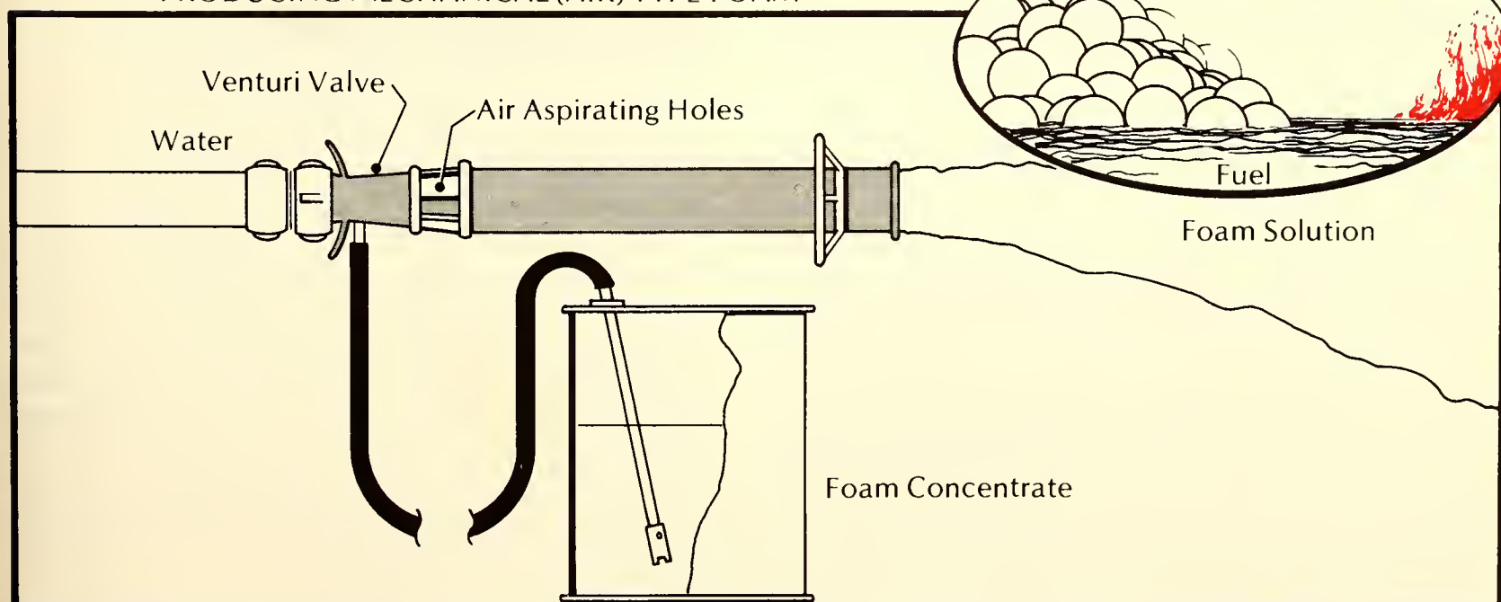
Figure 7.16. Production of mechanical (air) foam by mixing foam concentrate with water and air.
