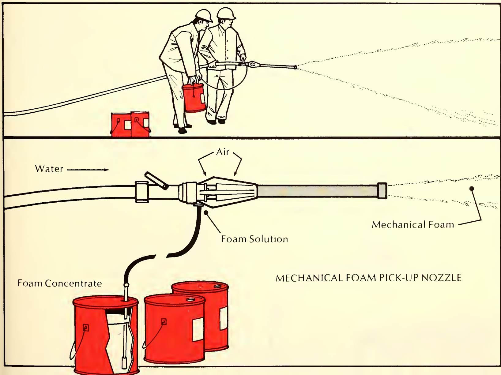
Figure 8.20. How foam is produced by the mechanical foam nozzle with pickup. The nozzle itself is a very efficient foam producer. However, the nozzleman's movements are restricted by the need to keep the pickup tube in the foam-concentrate container.
