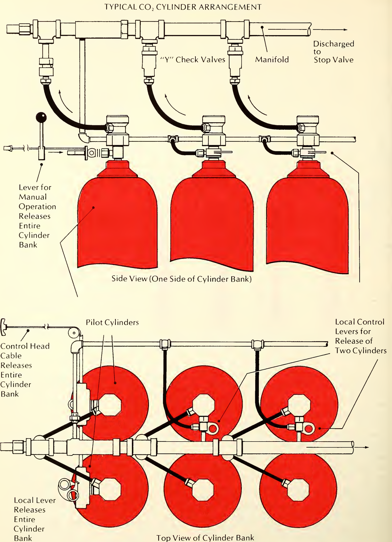
Figure 9.23. The pilot CO 2 cylinders must be activated last when CO 2 is routed to a cargo space fire. Otherwise, all the cylinders in the bank will be opened at once. (Courtesy Walter Kidde and Company)
