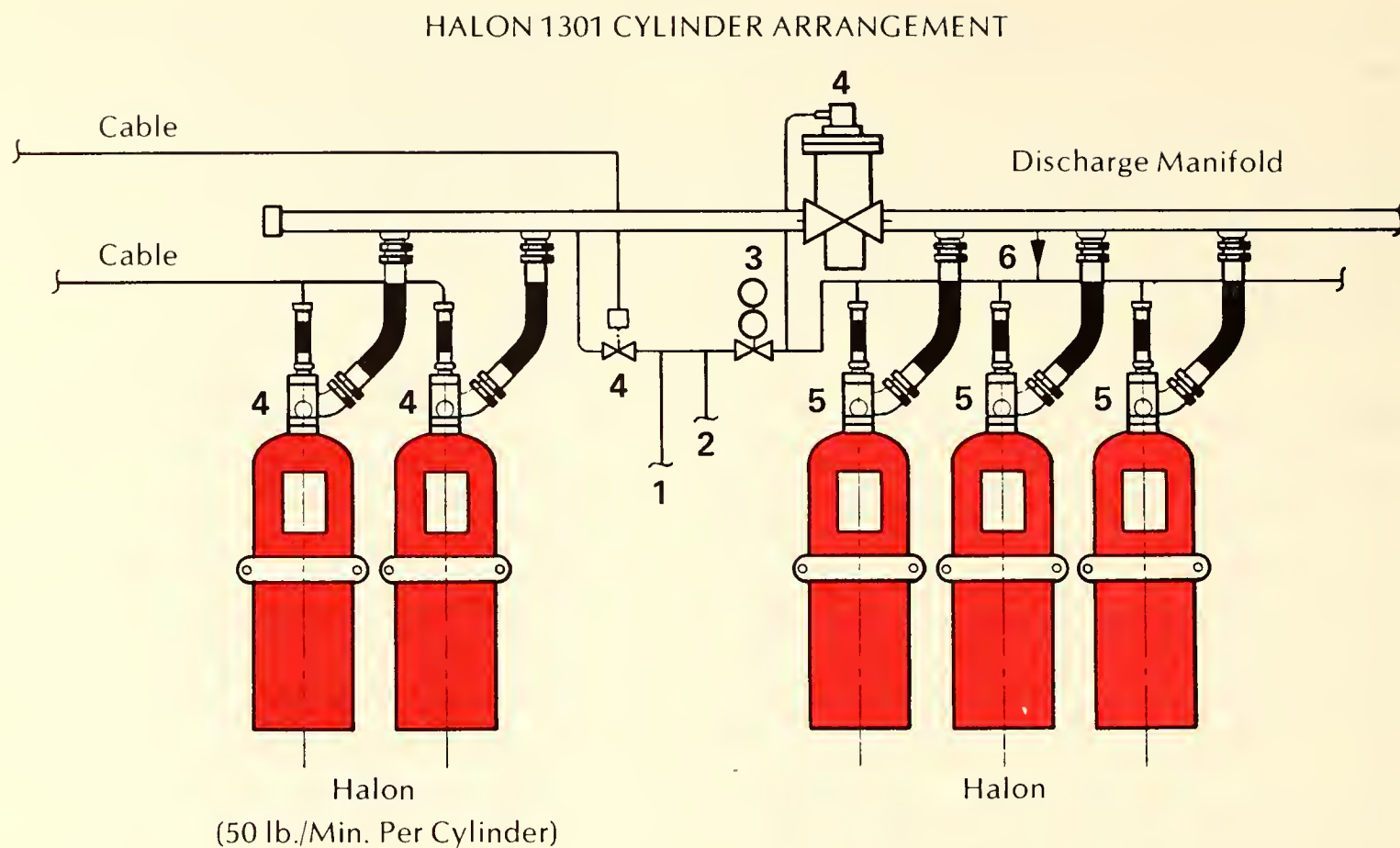
Figure 9.25. A U.S. Coast Guard approved arrangement for Halon 1301 cylinders in a manually operated engineered extinguishing system. 1) Line to pressure-operated alarm. 2) Line to pressure-operated switches. 3) Time delay. 4) Valve capable of manual operations. 5) Pressure-operated valve (cannot be operated manually). 6) Check valve.
