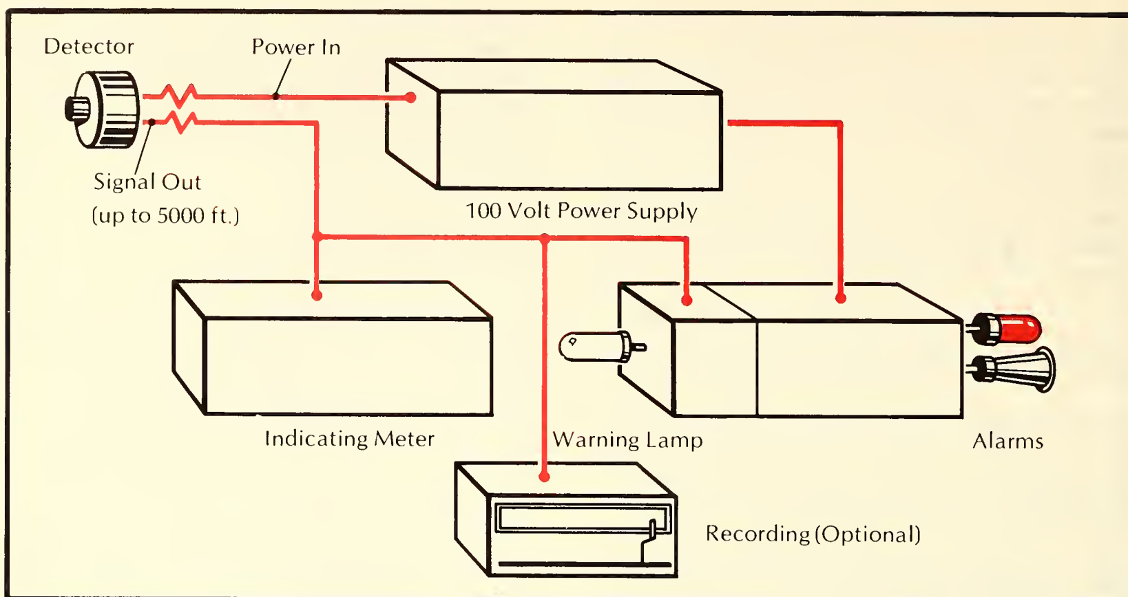
Figure 6.15. Schematic drawing of a catalytic combustible gas detection system.
