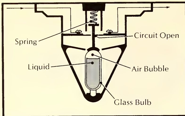
Figure 6.5A. The liquid expansion bulb. At normal temperatures, the bulb holds back the spring-loaded plunger.
