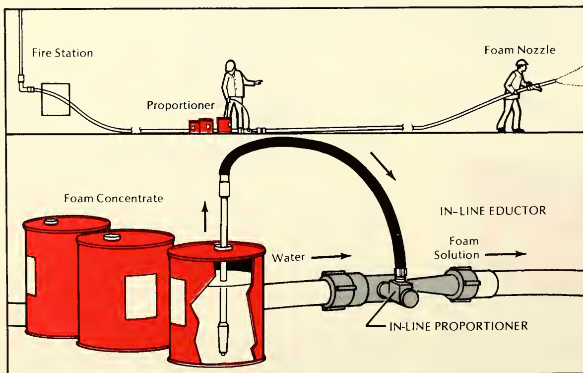
Figure 8.21. Production of mechanical foam by an in-line proportioner, or educator. The proportioner can be placed in the hoseline away from the fire, so the nozzleman has more mobility.
