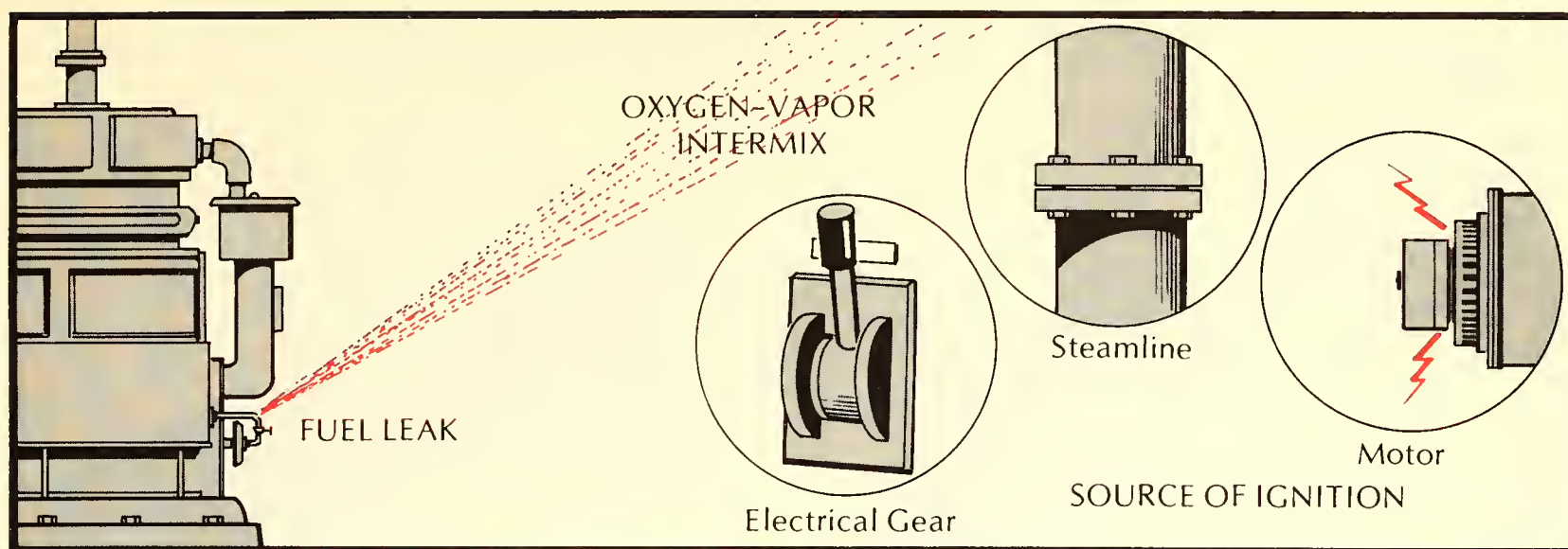
Figure 1.12. Fuel line leaks can spray vaporized fuel far enough to be ignited by steam lines or electrical equipment.
