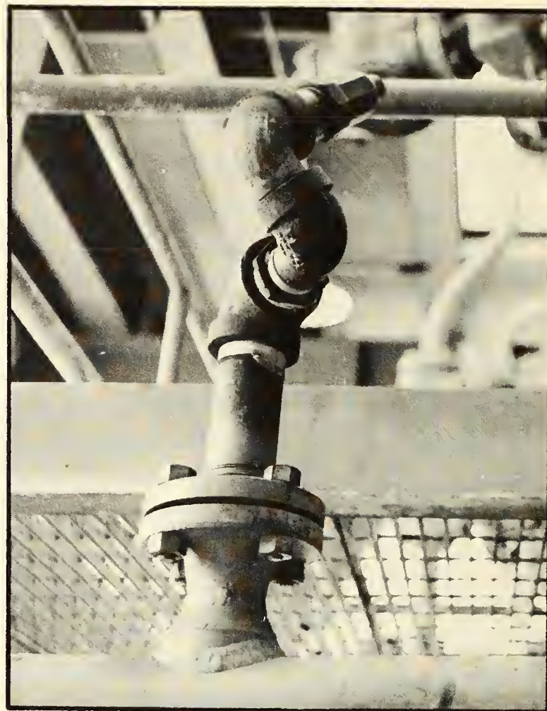
Figure 12.5. A spray nozzle primed to discharge a large volume of water into the well head area in case of fire.
