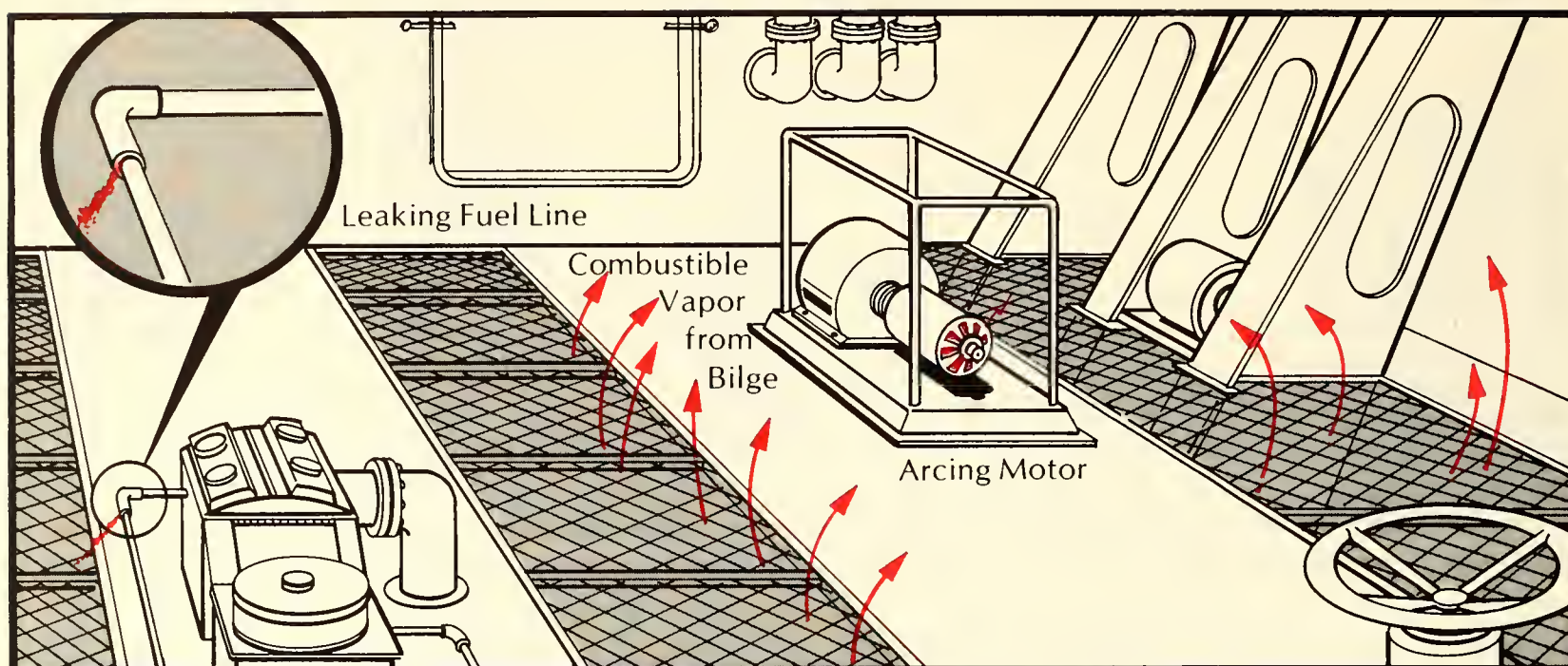
Figure 1.13. A disastrous combination not uncommon on vessels: Fuel from a leaking line collects in the bilge. Combustible fuel vapors from the bilge mix with air as they move toward the arcing motor. Ignition of the fumes by the motor can cause an explosion followed by fire.
