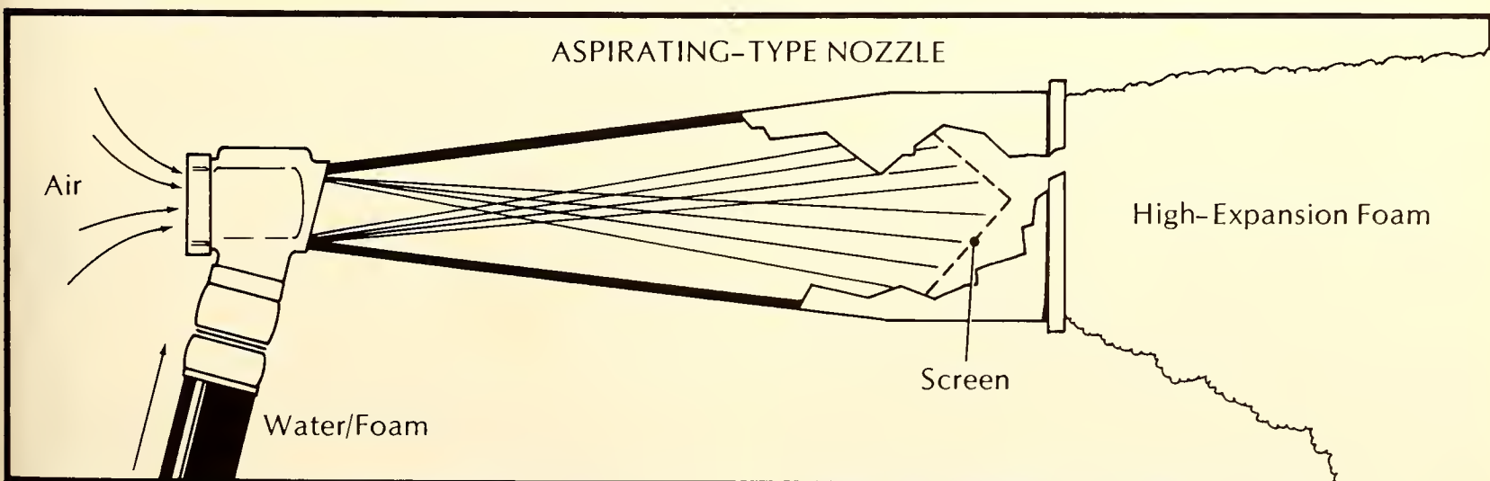
Figure 7.19. Production of high-expansion foam. High-velocity air strikes the water-foam concentrate solution at the screen, producing the foam.
