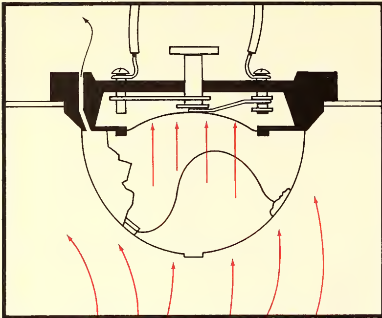
Figure 6.8A. Combined heat-actuated detector. The rate-of-rise device is a diaphragm that is stretched upward to close the contacts, when heat increases the pressure in the shell.
