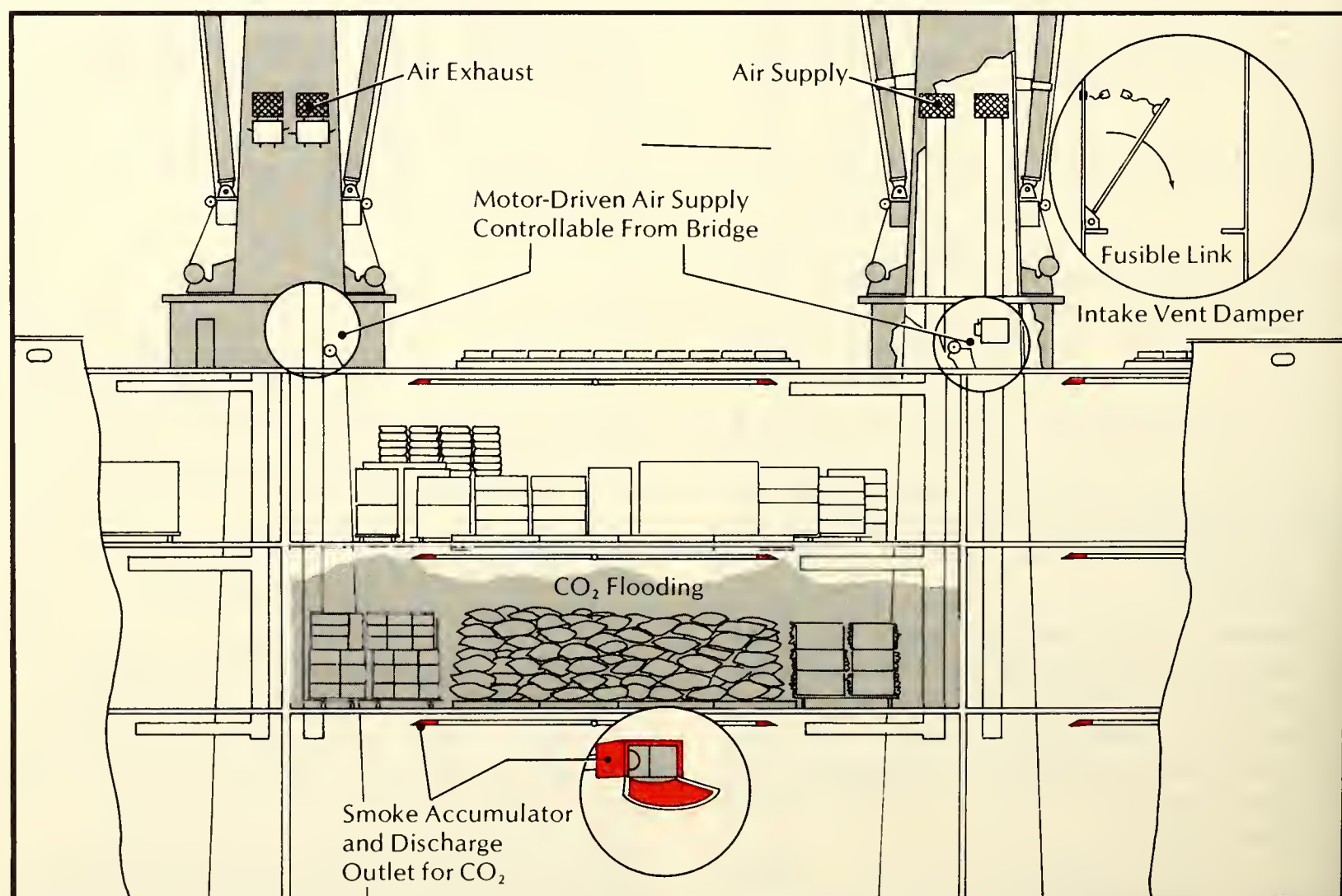
Figure 10.15. Cargo hold layout.
