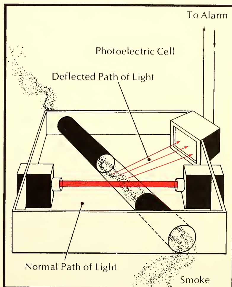
Figure 6.10. Refraction-type photoelectric smoke detector. Smoke in the air causes light to fall on the photoelectric sensor, which then activates the alarm.
