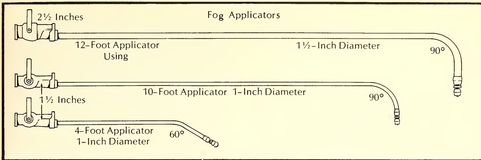
Figure 7.12. Low-velocity fog applicators approved for shipboard use.
