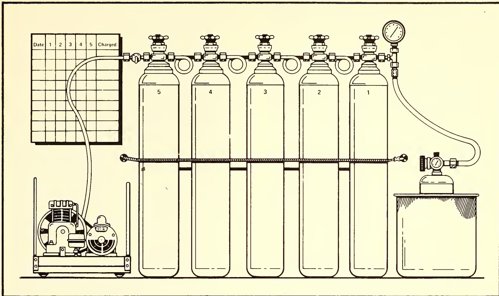
Figure 15.18. Cascaded air tanks for refilling breathing apparatus cylinders.
