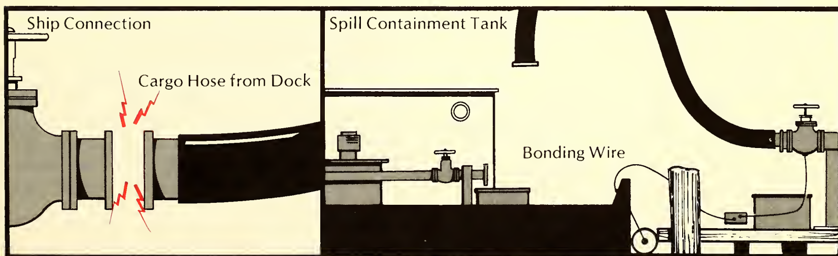
Figure 1.16. An electrical bond between the vessel and the shoreside facility (right) prevents sparks caused by static electricity (left). The bonding should be completed before the cargo hose is connected to the shore connector.
