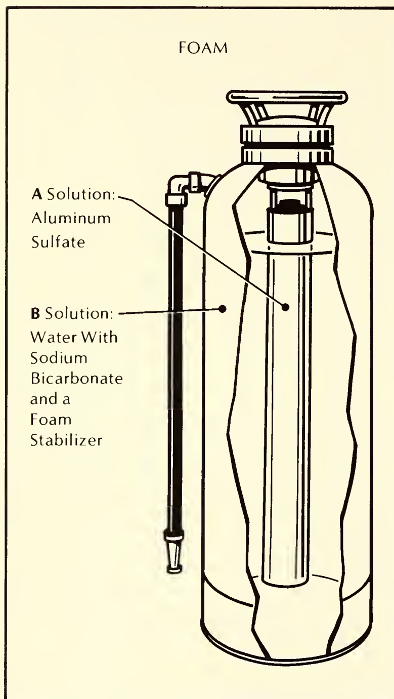
Figure 8.6. Cutaway of foam extinguisher used for class A and class B fires showing
