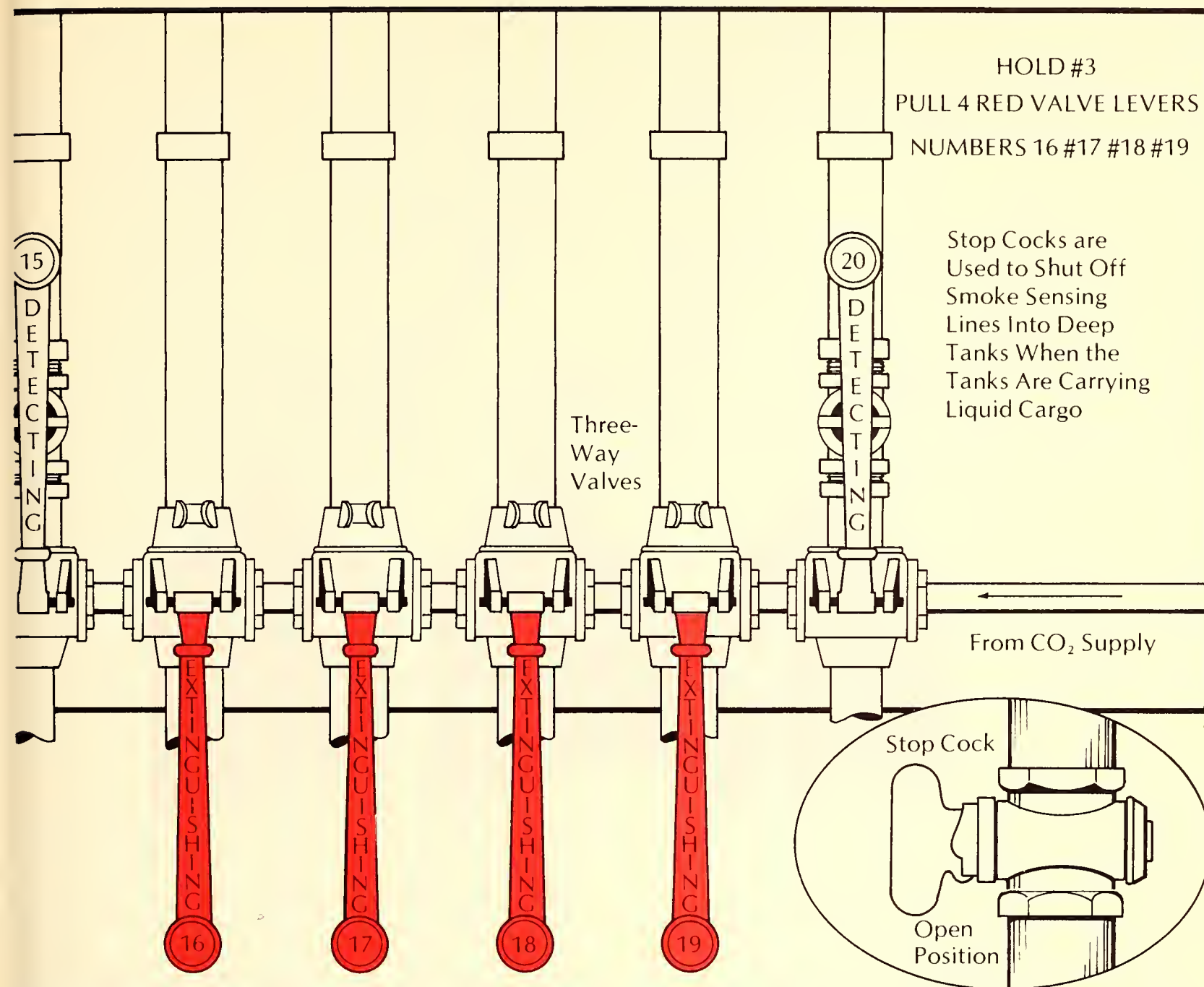
Figure 9.22. The proper three-way valve (or valves) must be pulled down to route CO 2 to the involved space. Here, the involved space is served by four lines.
