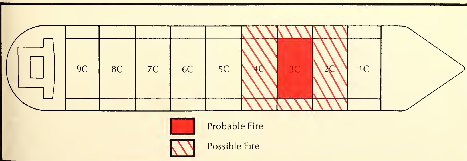
Figure 9.19. Tanker configuration used to determine the required rate of foam flow.
