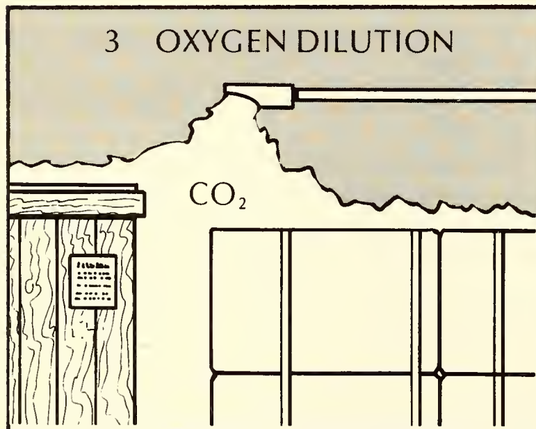
Figure 7.1. A. Cooling agents absorb heat from the fire. B. Smothering agents separate the fuel from its oxygen supply. C. Oxygen diluting agents reduce the amount of oxygen available. D. Chain breakers attack the chemical process that keep the fire going.
