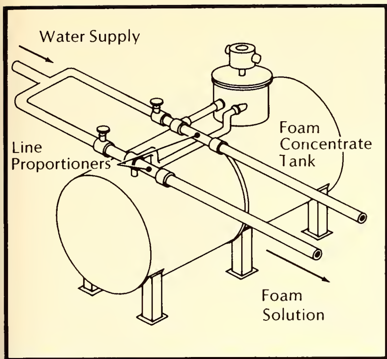
Figure 9.17. Venturi-affect foam tank with dual proportioners. This type of tank does not require a separate foam concentrate pump. (Courtesy National Foam System, Inc.)
