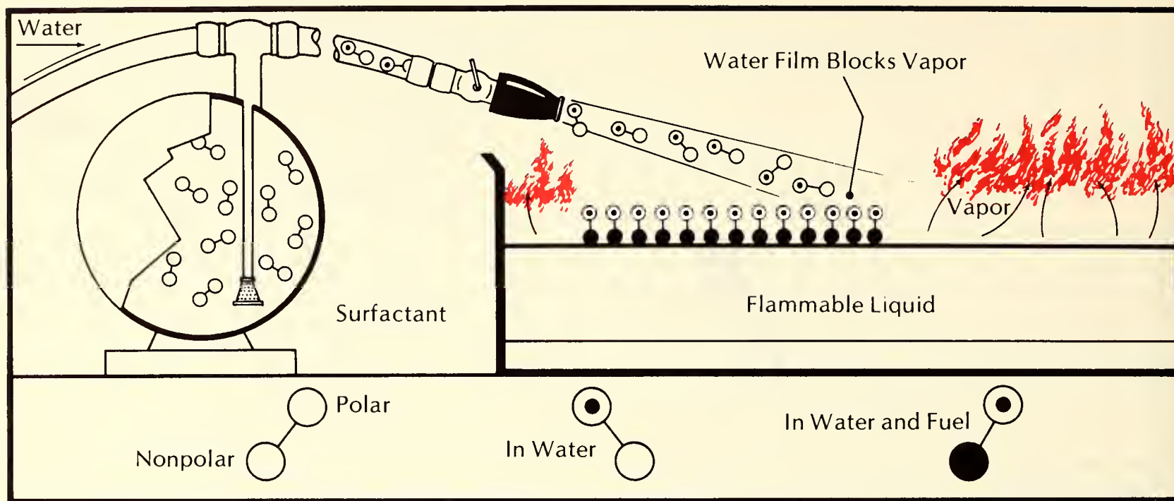
Figure 7.17. The AFFF surfactant molecule holds water at one end and flammable liquid fuel at the other end. It thus forms a thin layer of water on top of the burning fuel.
