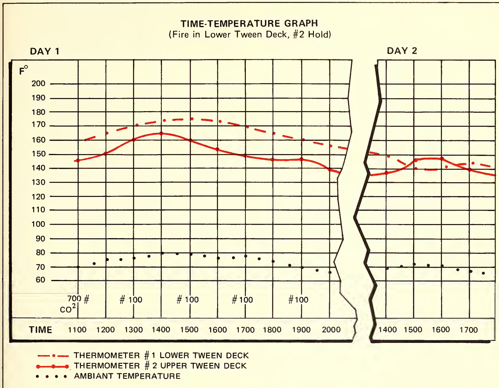
Figure 10.16. Temperature graph for recording information regarding an indirect attack on a hold fire with the CO 2 total-flooding system.
