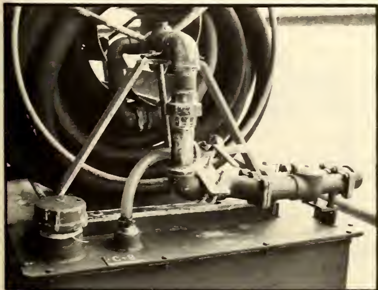
Figure 12.9. Some fire stations have a foam concentrate storage tank as an integral part of the fire-main system. By opening the eductor valve the hoseline is supplied with a foam solution.
