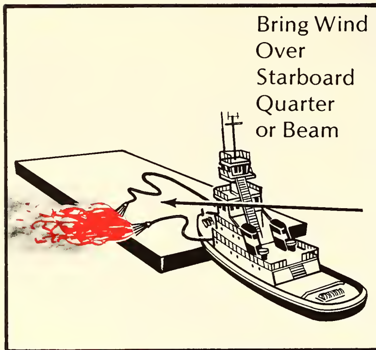
Figure 11.13. When the barge fire is near the tug, the barge should be maneuvered so the wind pushes the fire away from the tug and toward the shortest paths of possible fire travel.
