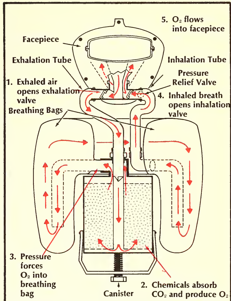
Figure 15.8. The numbers show the sequence of events during one operating cycle of the canister-type OBA. The arrows show the flow of exhaled breath and inhaled oxygen.
