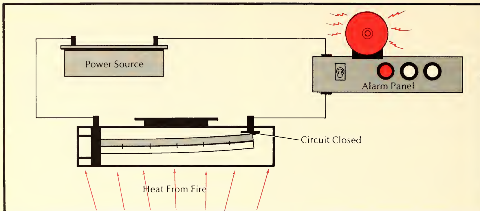
Figure 6.1B. As temperature rises, the strip bends upward, because the lower metal expands more than the upper metal. At temperatures within its activating range, the strip bends enough to touch the contact and complete the alarm circuit.
