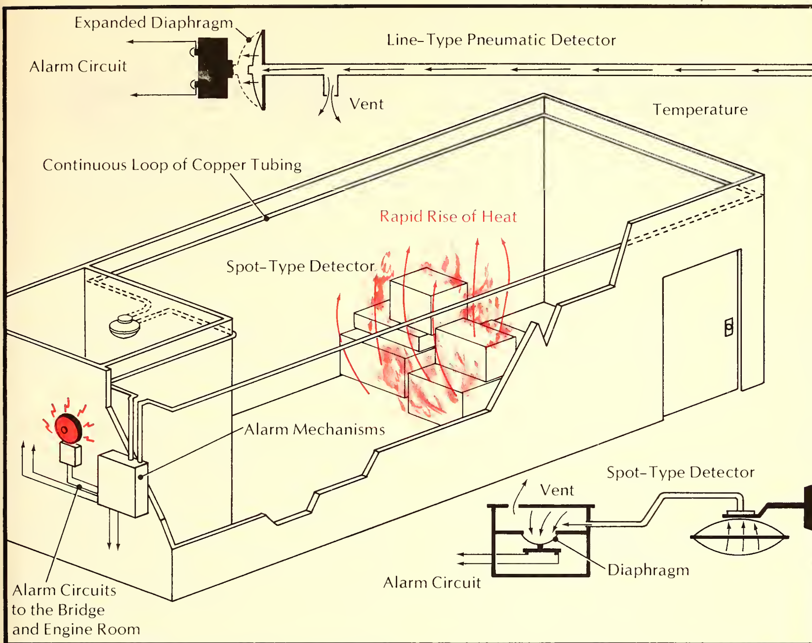
Figure 6.6. Pneumatic rate-of-rise detectors. Heat expands the air inside the tube or bulb, increasing its pressure. If the expansion is slow, the vent releases enough of the pressure to keep the detector from being actuated. If the expansion is fast, pressure builds up enough to stretch the diaphragm and complete the alarm circuit.
