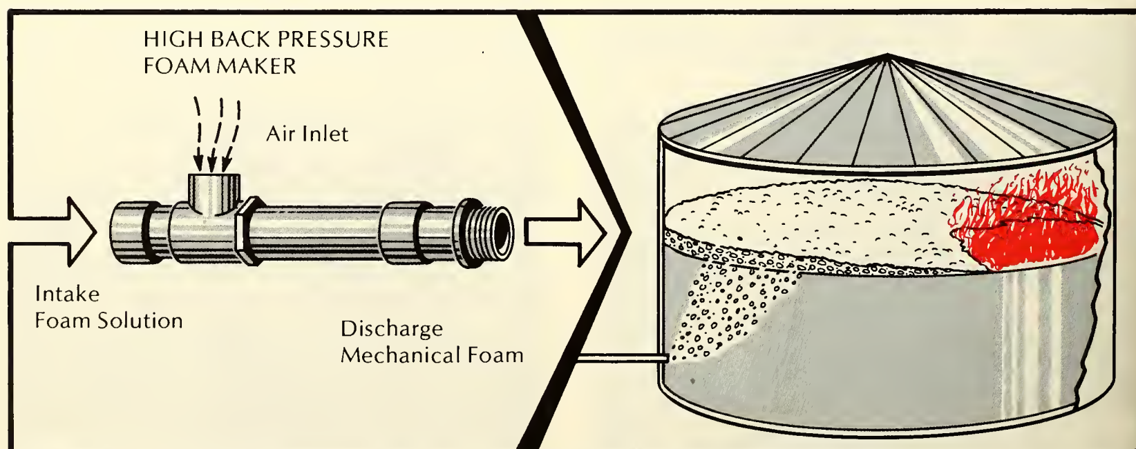
Figure 12.11. In the subsurface foam injection system, mechanical foam is forced up through the contents in the tank to form a floating blanket that smothers the fire.
