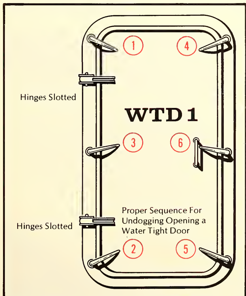
Figure 16.1. The numbers show the proper sequence for releasing the dogs on a watertight class 1 door.
