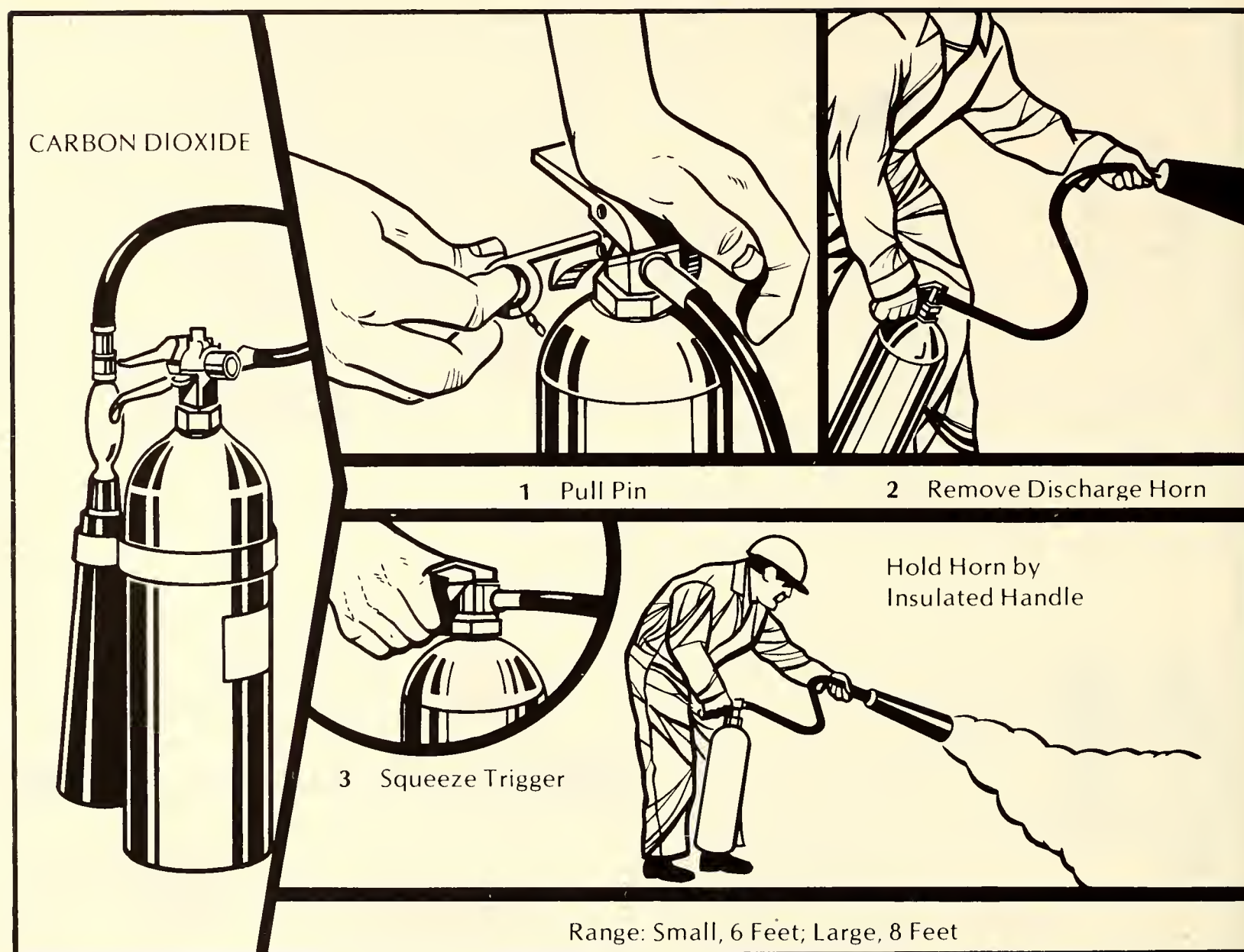
Figure 8.8A. Steps in operating the CO 2 extinguisher used for class B and class C fires.
