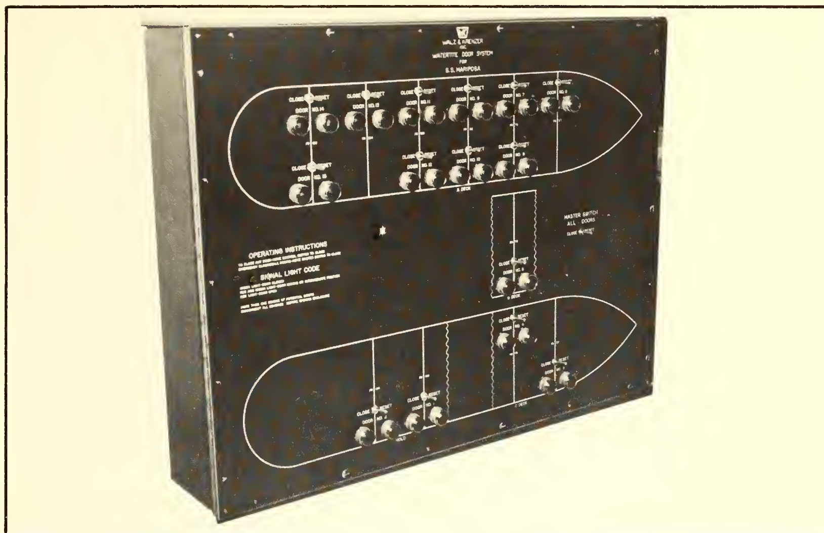
Figure 16.3. Central control station for watertight doors. (Courtesy Walz and Krenzer Inc.)
