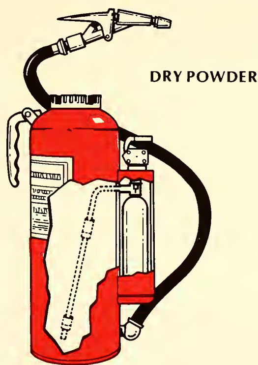
Figure 8.11. Dry-powder extinguisher used for class D fires only.
