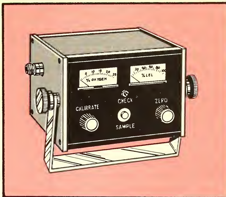
Figure 16.7. Combination portable combustible gas and oxygen indicator. (Courtesy Mine Safety Appliances Company)
