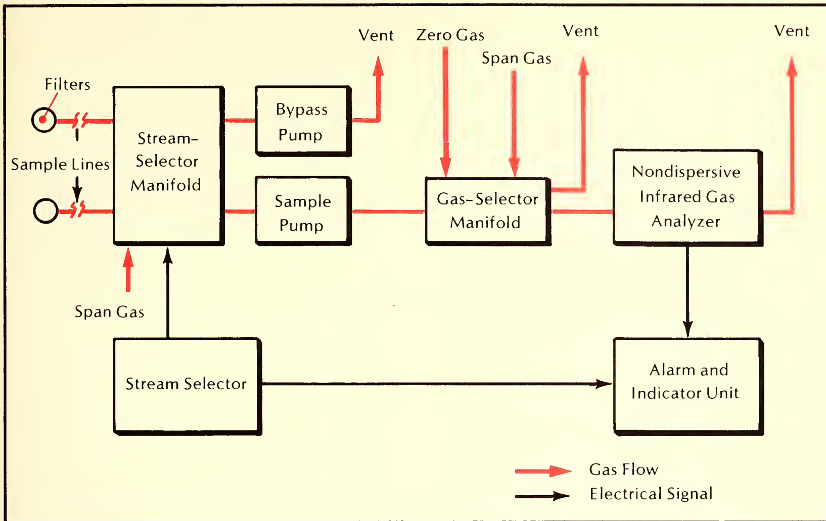
Figure 6.16. The main components of an infrared shipboard gas-monitoring system. (Courtesy Beckman Instruments, Inc., Mountainside, N.J.)
